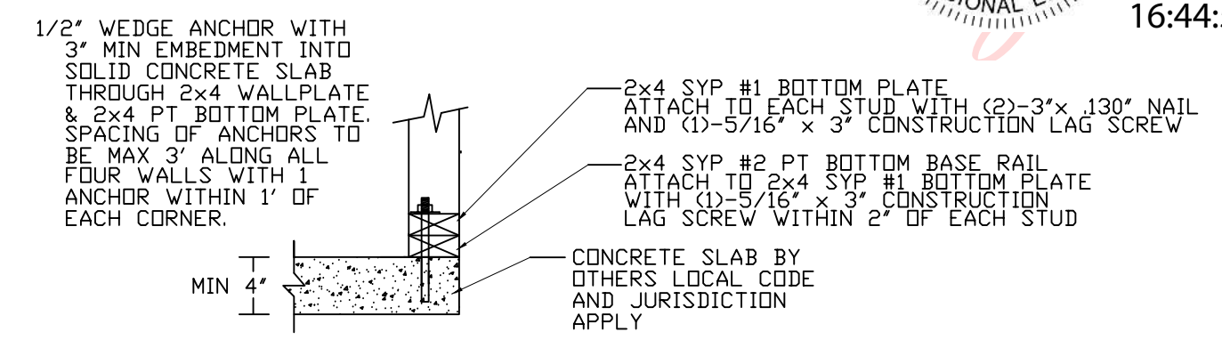
SHED WITHOUT FLOOR ANCHORED TO CONCRETE END VIEW
