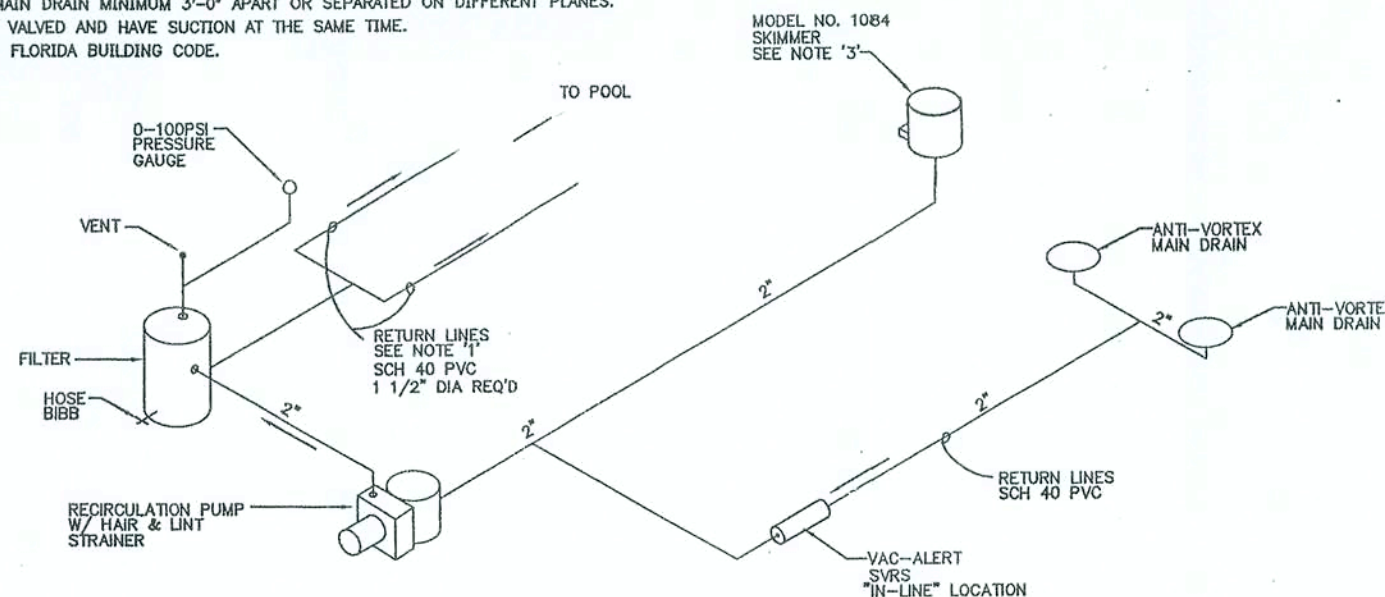
VAC-ALERT OPTION NTS
