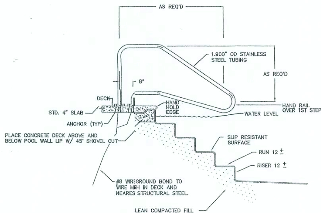
STP HANDRAIL SECTION NOT TO SCALE
