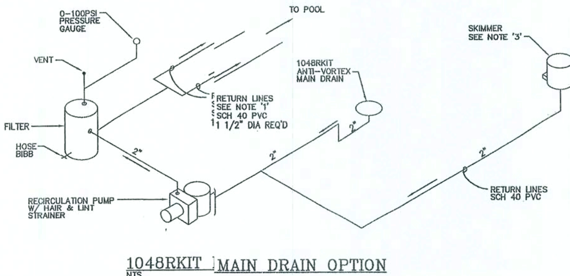
1048RKIT MAIN DRAIN OPTION NTS
