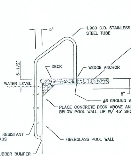
LADDER SECTION NOT TO SCALE
