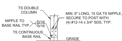
2B POST/BASE RAIL CONNECTION SCALE: NTS
