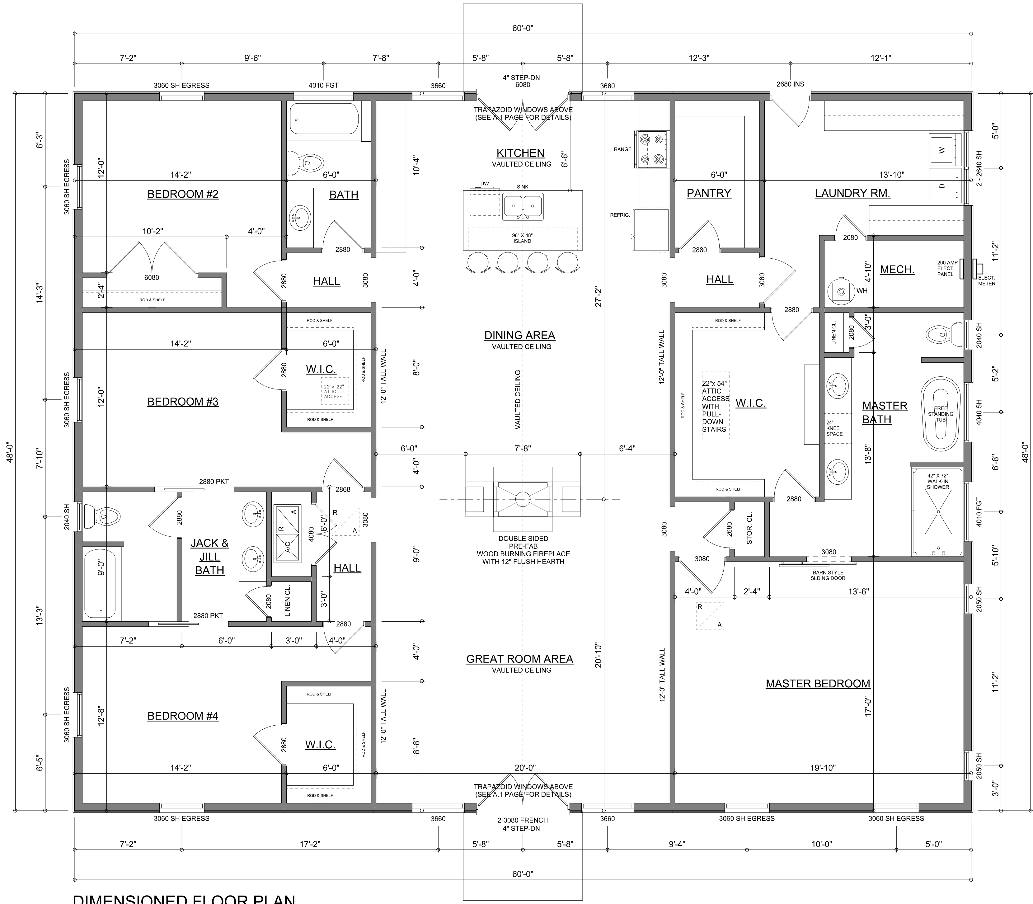
DIMENSIONED FLOOR PLAN SCALE: 1/4" = 1'-0" NOTE: ALL WALLS SHALL BE 10'-0" UNLESS OTHERWISE NOTED.
