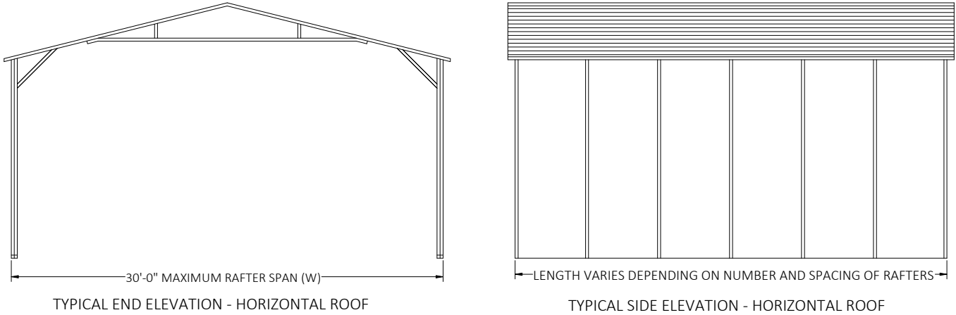
BOX EAVE FRAME RAFTER OPEN BUILDING
