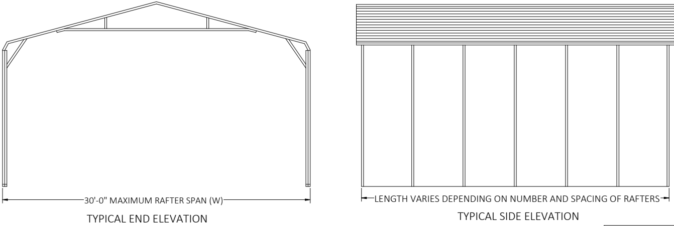
BOW FRAME RAFTER OPEN BUILDING
