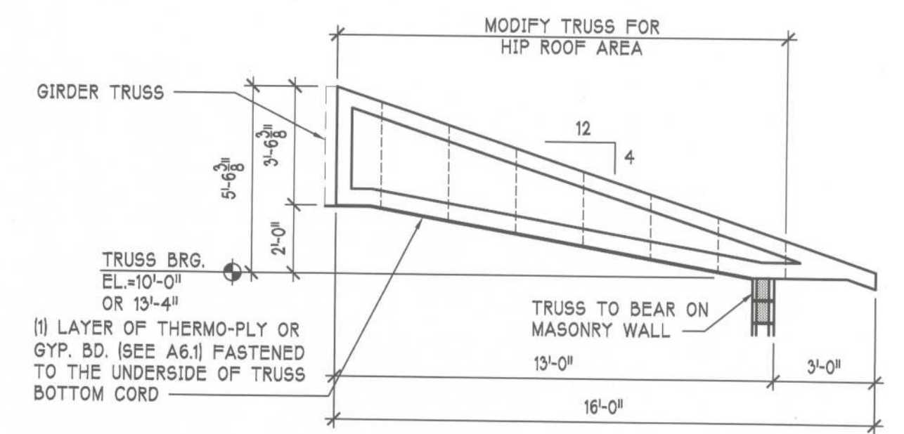
T6 - TRUSS
