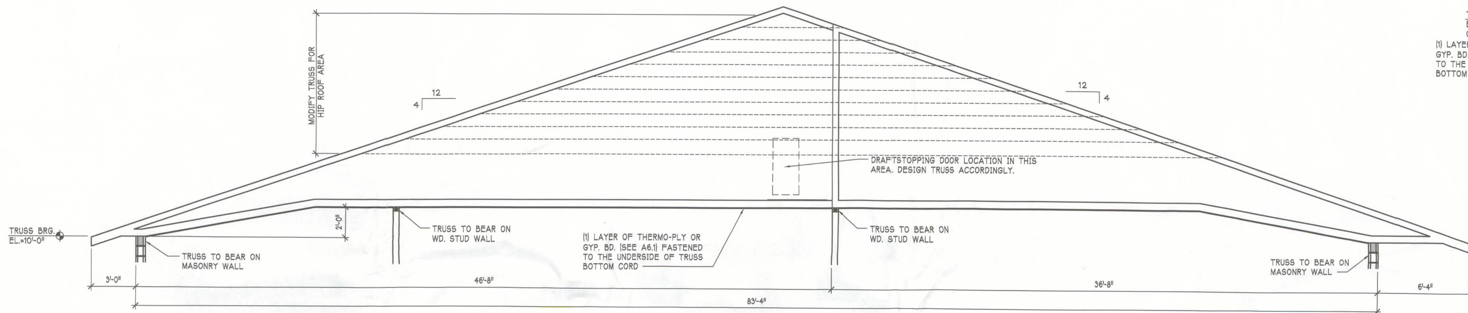
T2 - TRUSS
