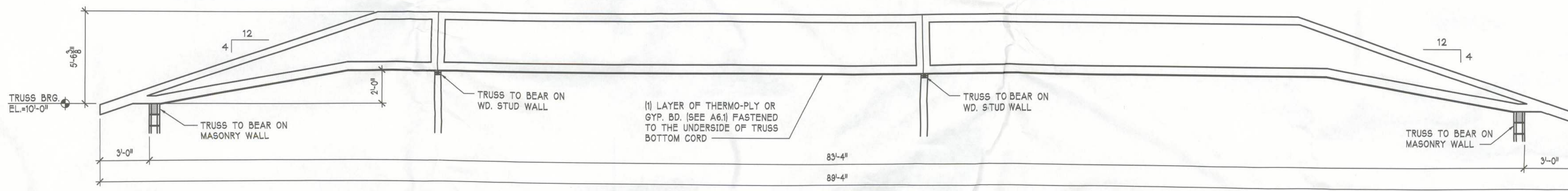
T3 - GIRDER TRUSS
