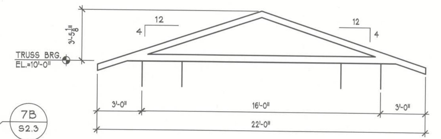
T5 - TRUSS
