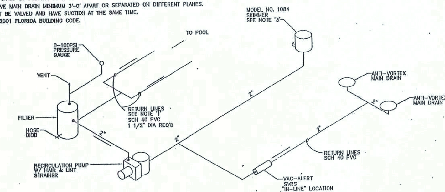
VAC-ALERT OPTION NTS
