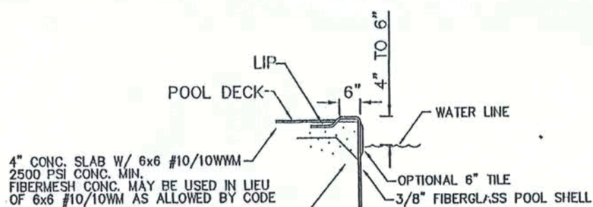
ALTERNATE COPING DETAIL NOT TO SCALE
