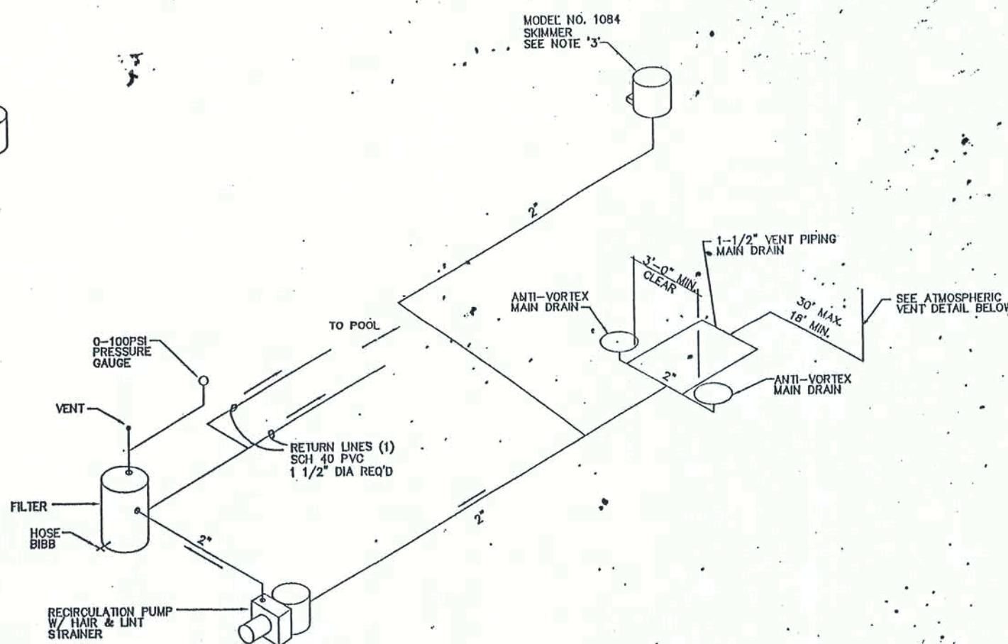
ATMOSPHERIC VENT OPTION NTS
