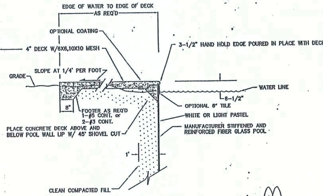
WALL SECTION NOT TO SCALE
