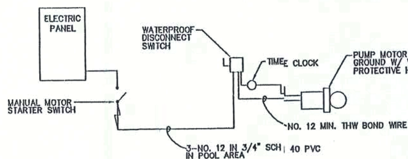
ELECTRICAL DIAGRAM NTS
