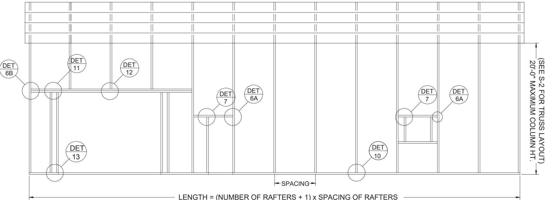
LENGTH = (NUMBER OF RAFTERS + 1) x SPACING OF RAFTERS SPACING = 5'-0" FOR WIND SPEEDS BETWEEN 110 MPH AND 140 MPH SPACING = 4'-0" FOR WIND SPEEDS BETWEEN 140 MPH AND 180 MPH TYPICAL BOX EAVE RAFTER SIDE FRAMING SECTION SCALE: NTS
