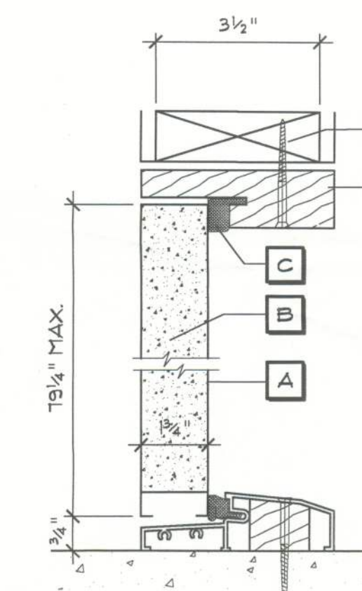
TYPICAL VERTICAL SECTION
