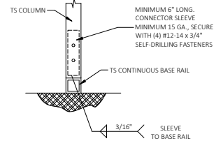
2 RAFTER POST/BASE RAIL CONNECTION DETAIL SCALE: NTS
