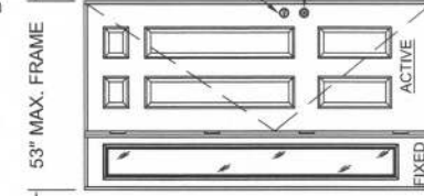
4-2 X 8-0 ELEVATION
