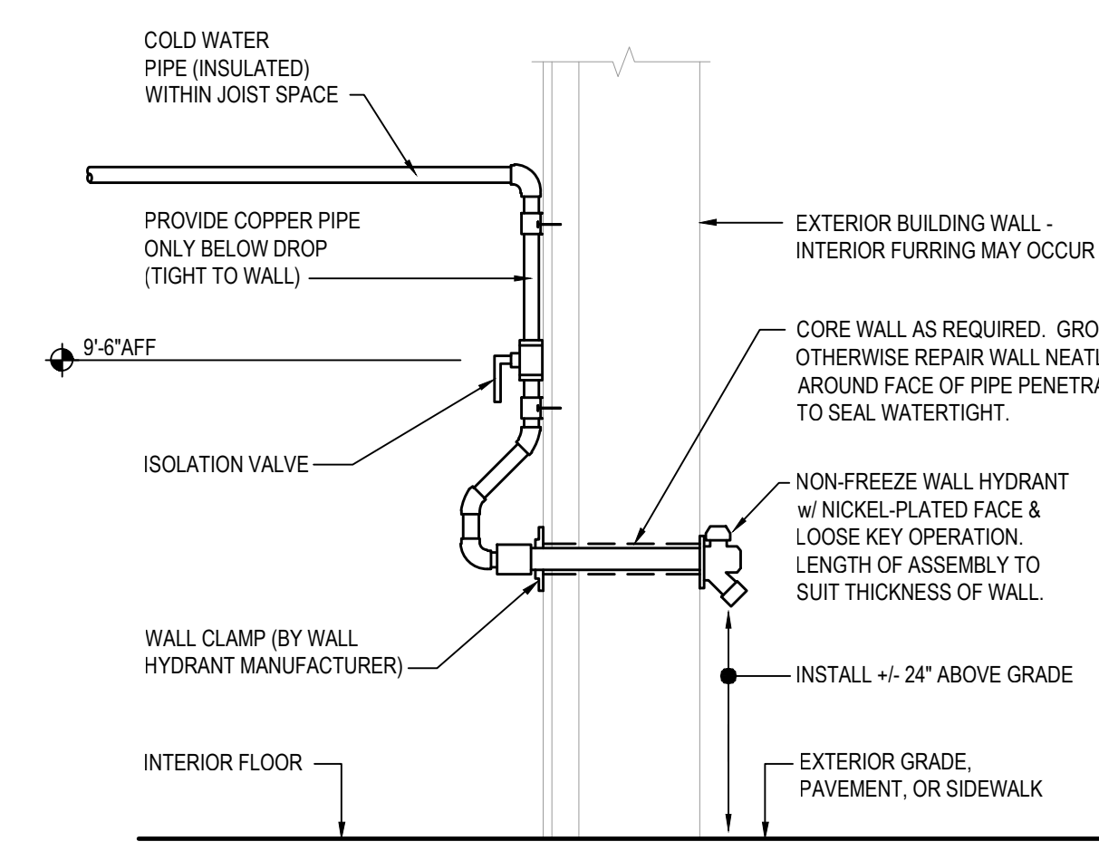
5 | WALL HYDRANT DETAIL (HB1) N.T.S.
