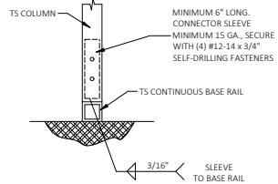
2 RAFTER POST/BASE RAIL CONNECTION DETAIL SCALE: NTS
