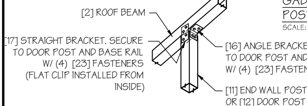
END WALL POST - ROOF BEAM CONN. DETAIL
