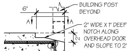
OVERHEAD DOOR NOTCH DETAIL
