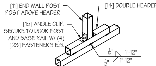
GABLE BRACE - END WALL CONN. DETAIL
