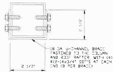
BRACE SECTION
