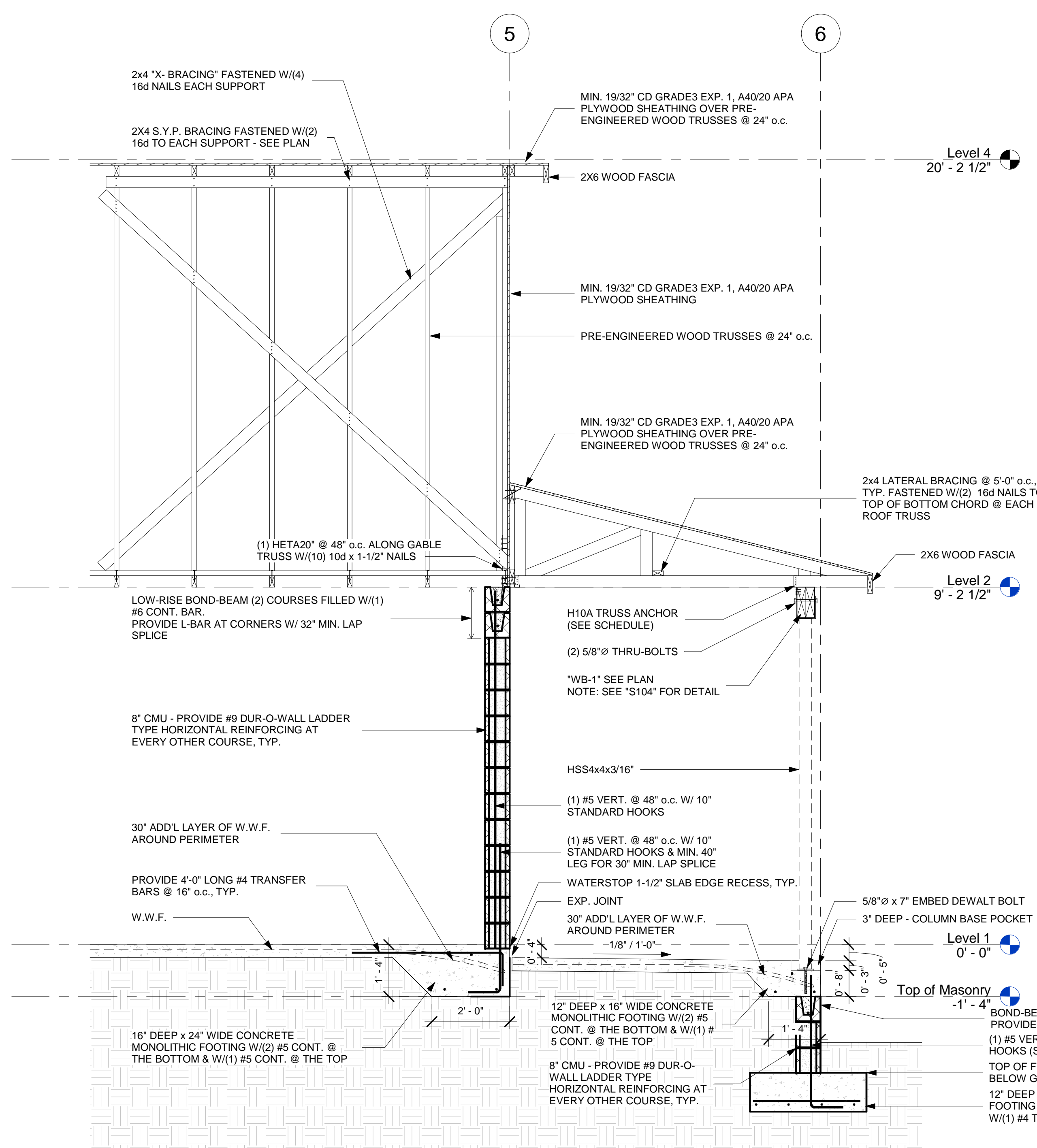
2 Structural Building Section 2 1/2" = 1'-0"
