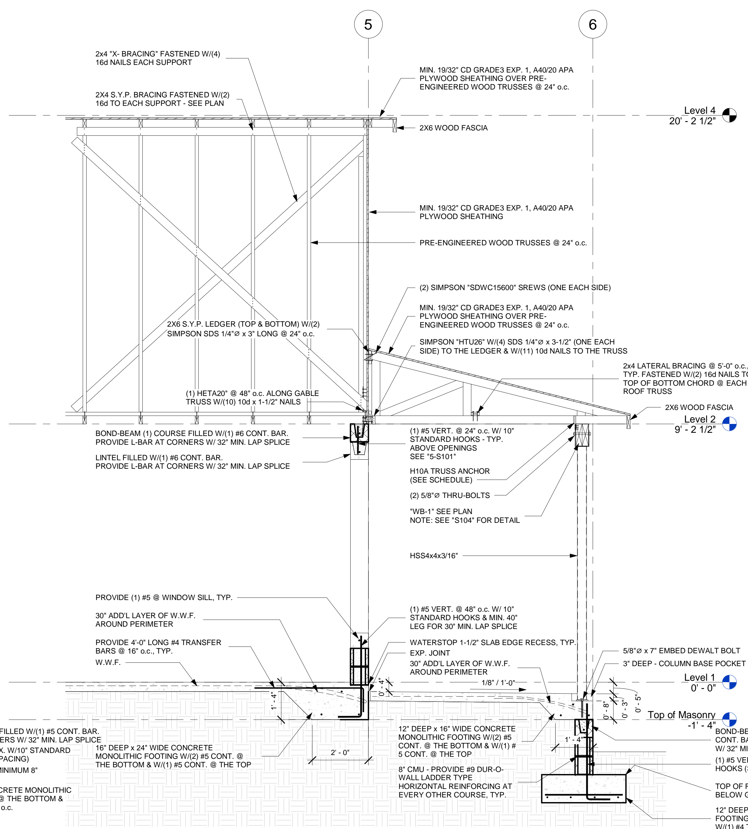
1 Structural Building Section 1 1/2" = 1'-0"
