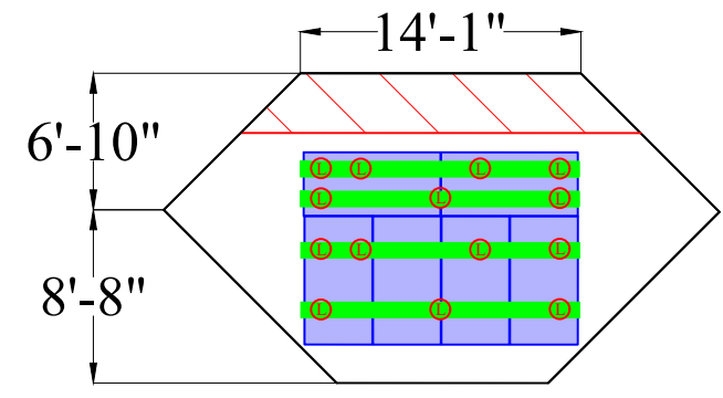
R-2 # Modules (6) Pitch: 25° Azimuth: 274°
