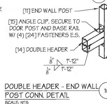
END WALL POST ABOVE DOUBLE HEADER CONN. DETAIL SCALE: NTS
