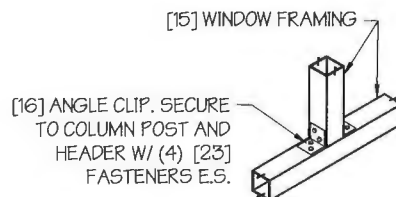
TYP. WINDOW FRAMING
