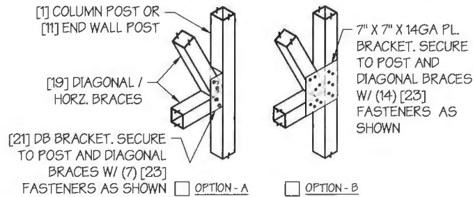
DIAGONAL BRACE - POST CONN. DETAIL* SCALE: NTS
