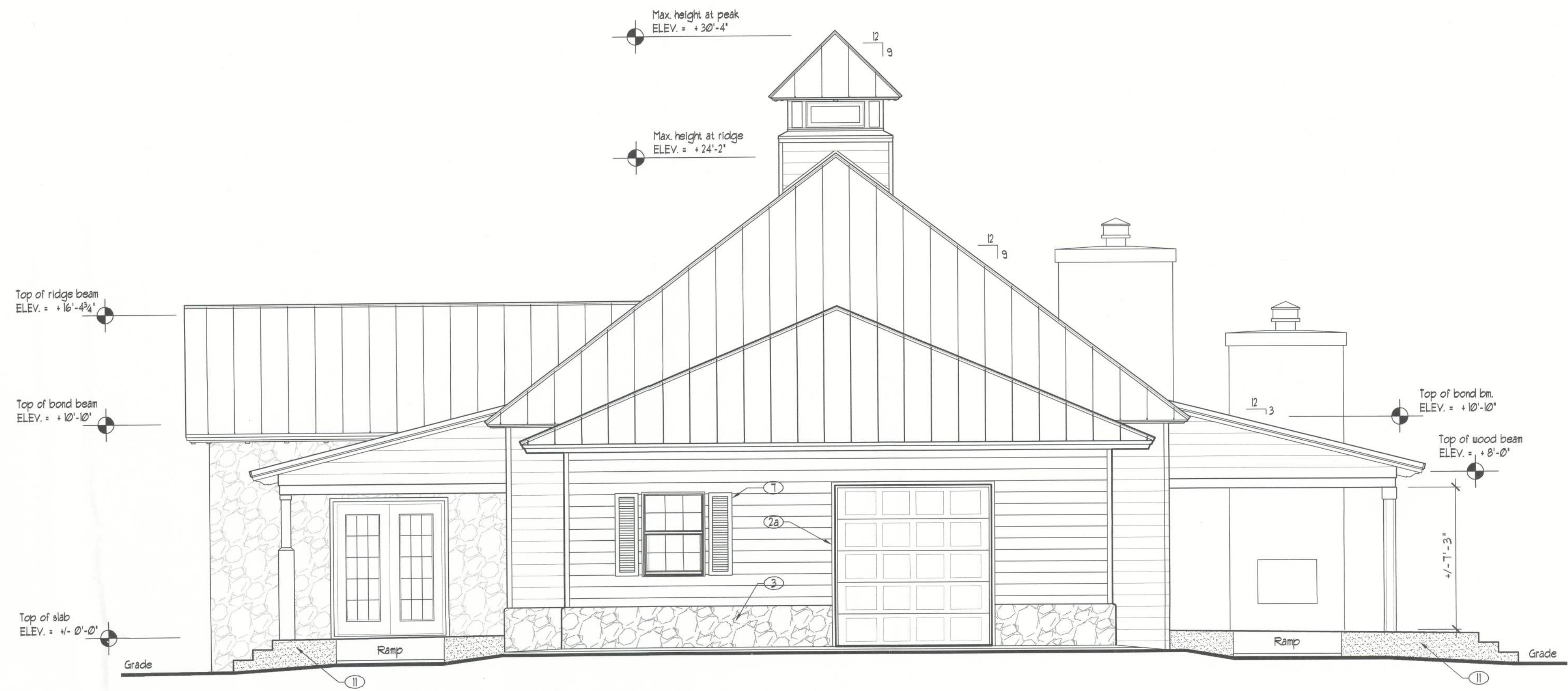
SOUTH RIGHT ELEVATION scale: 1/4" = 1'-0"
