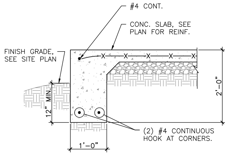
S 2 PERIMETER FOOTING
