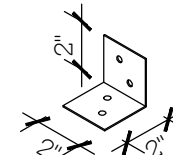
THICKNESS = 14GA ANGLE BRACKET SCALE: NT5
