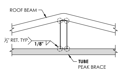
4 PEAK SUPPORT CONN. DETAIL SCALE: NTS
