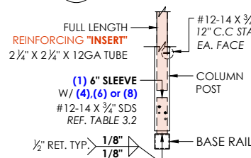
3 BASE CONN. DETAIL SCALE: NTS
