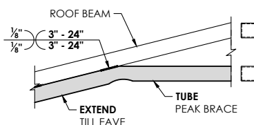
2 PEAK CONN. DETAIL SCALE: NTS
