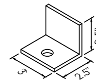
OPTION A 1 1/2" X 2 1/2" X 3/16" SCALE: NT5
