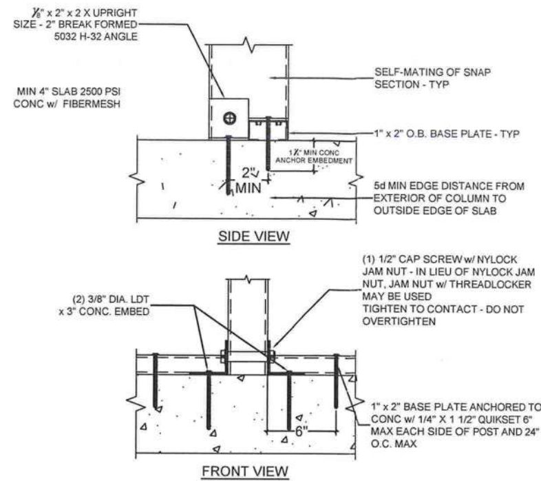
B A-2 2" x 4" OR LARGER SELF-MATING UPRIGHT TO DECK DETAILS SCALE: NTS
