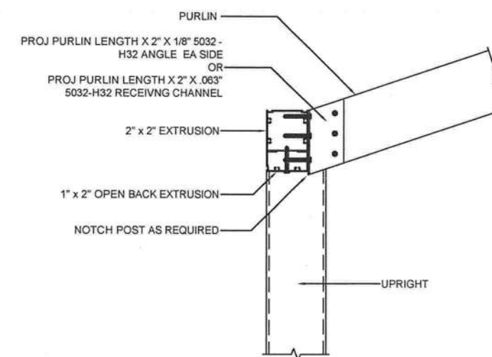
F A-2 SLOPED PURLIN CONNECTION DETAIL SCALE: NTS
