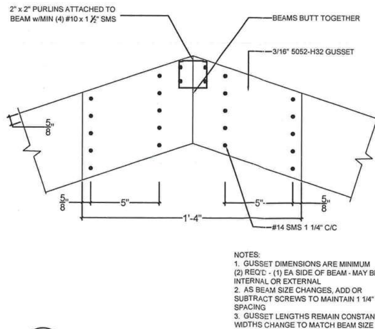
E A-2 TYPICAL INTERNAL OR EXTERNAL GUSSET DETAIL - RIGID MEDIUM SCALE: NTS
