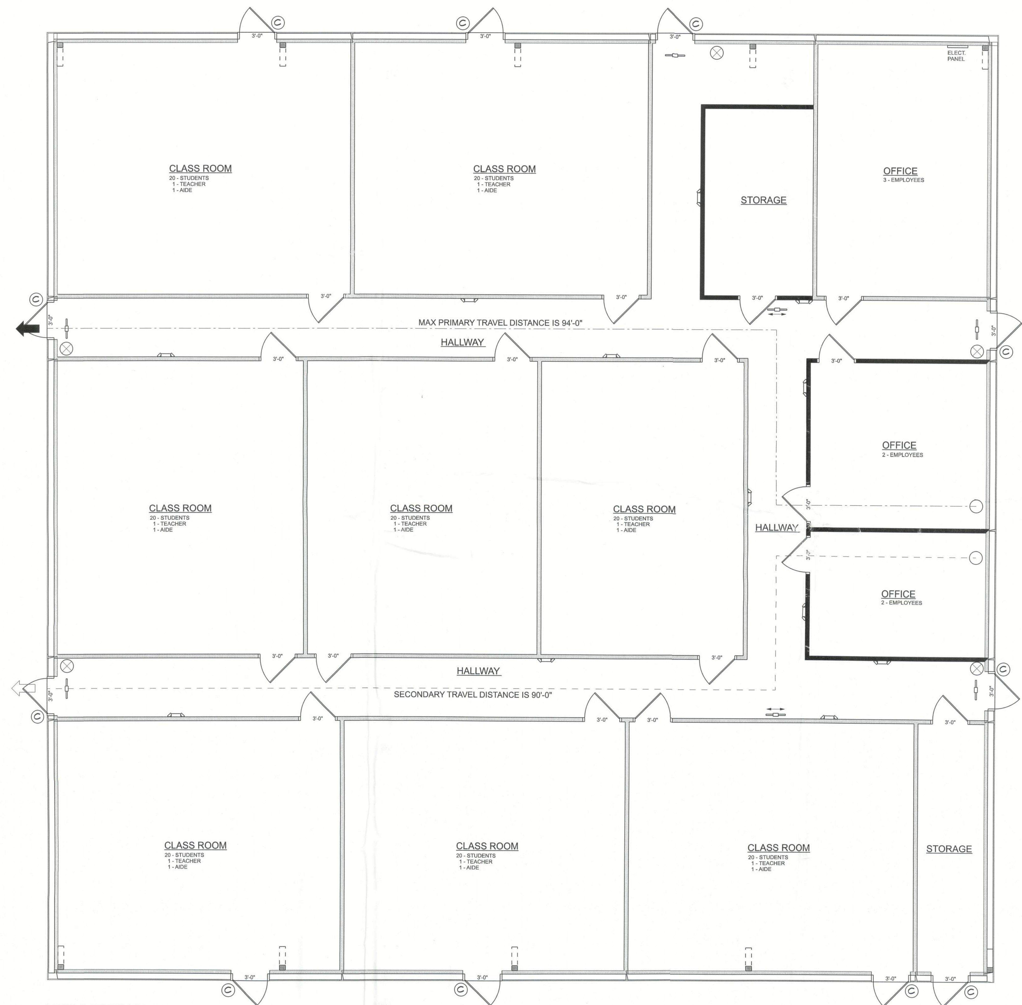
LIFE SAFETY PLAN SCALE: 1/4" = 1'-0"
