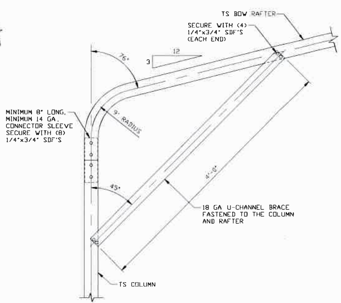
1B BOX EAVE RAFTER/CORNER POST CONNECTION DETAIL FOR HEIGHTS ≤ 12'-0" SCALE: NTS
