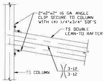
15 LEAN-TO RAFTER TO RAFTER POST CONNECTION DETAIL FOR WIDTHS 12'-0' < TO < 16'-0'
