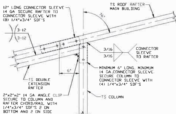
14 SIDE EXTENSION RAFTER/ COLUMN DETAIL FOR RAFTER SPANS 12'-0' < TO < 16'-0'
