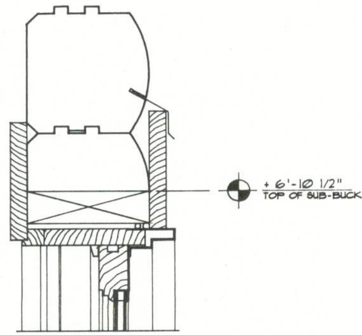
HEAD DET., 1/2 LOG STARTER
