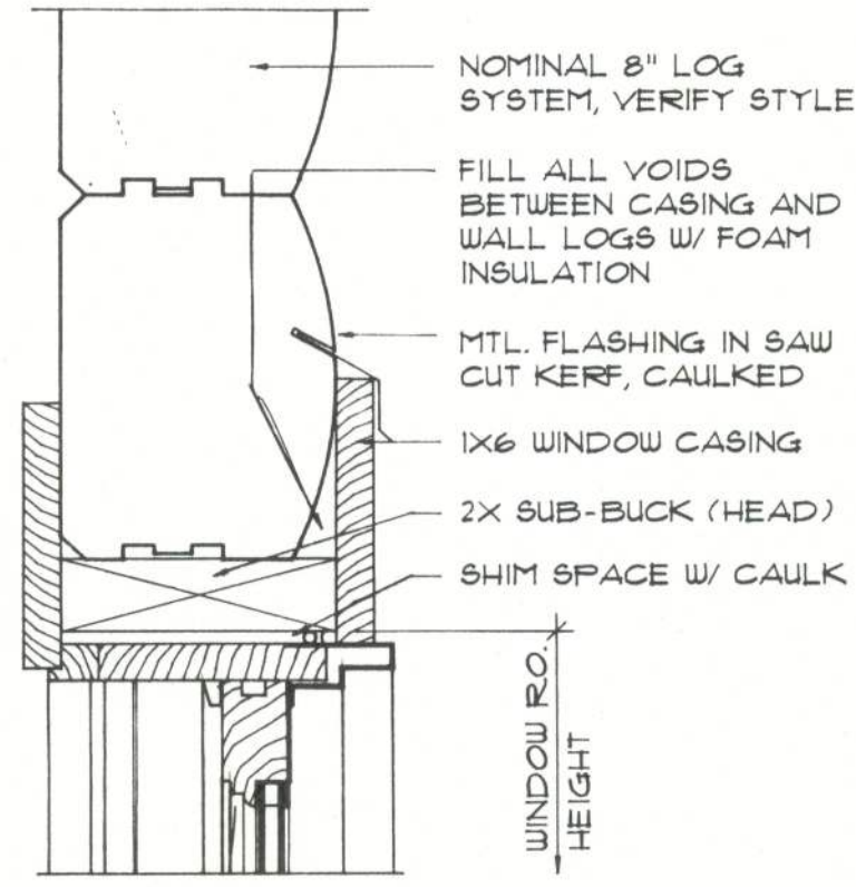
HEAD DET., FULL LOG STARTER
