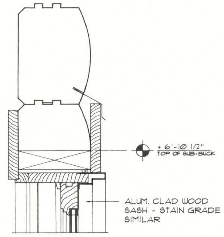
HEAD DET., 1/2 LOG STARTER
