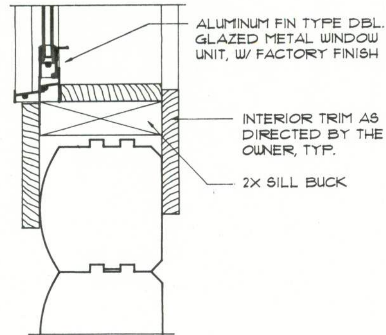
SILL DETAIL MTL. SASH
