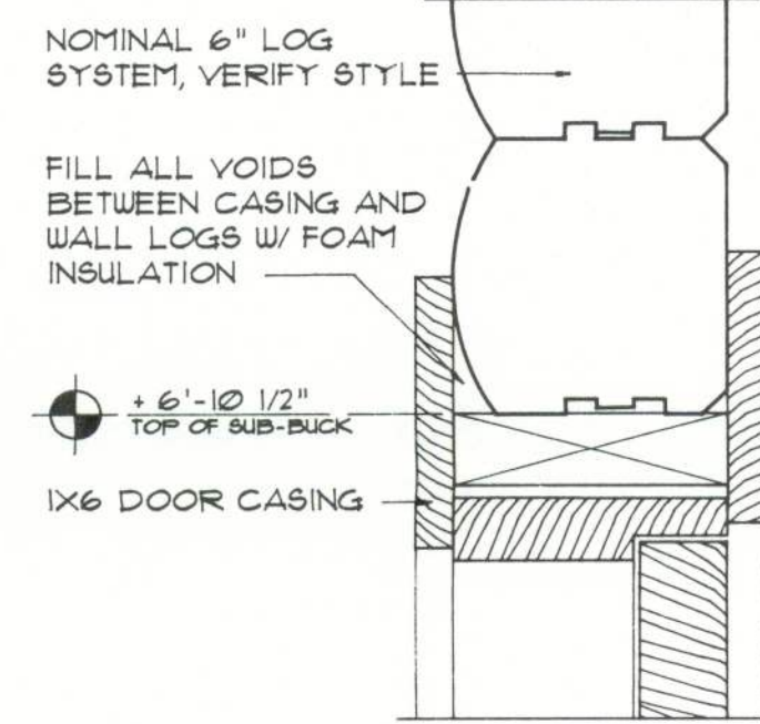
HEAD DETAIL DOOR
