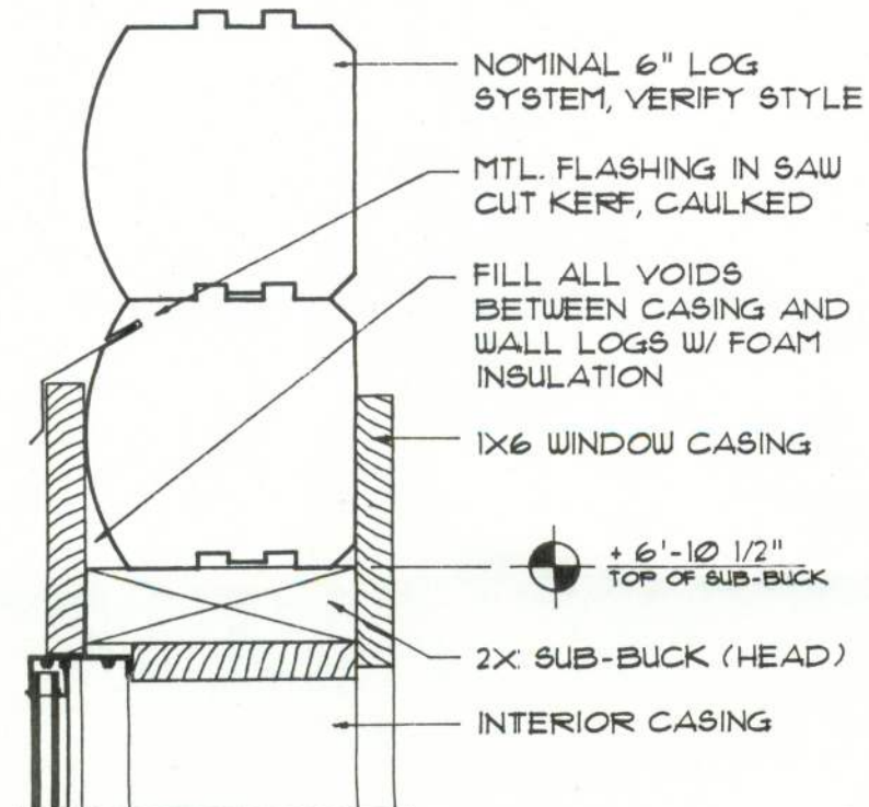
HEAD DETAIL MTL. SASH
