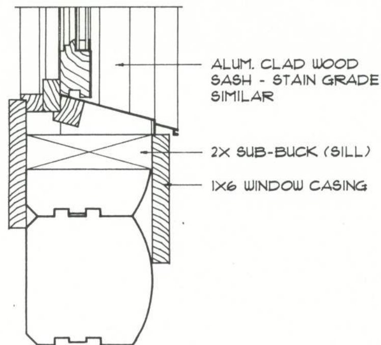
SILL DETAIL WOOD SASH
