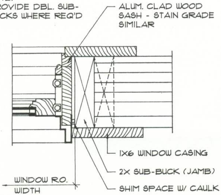
JAMB DETAIL WOOD SASH
