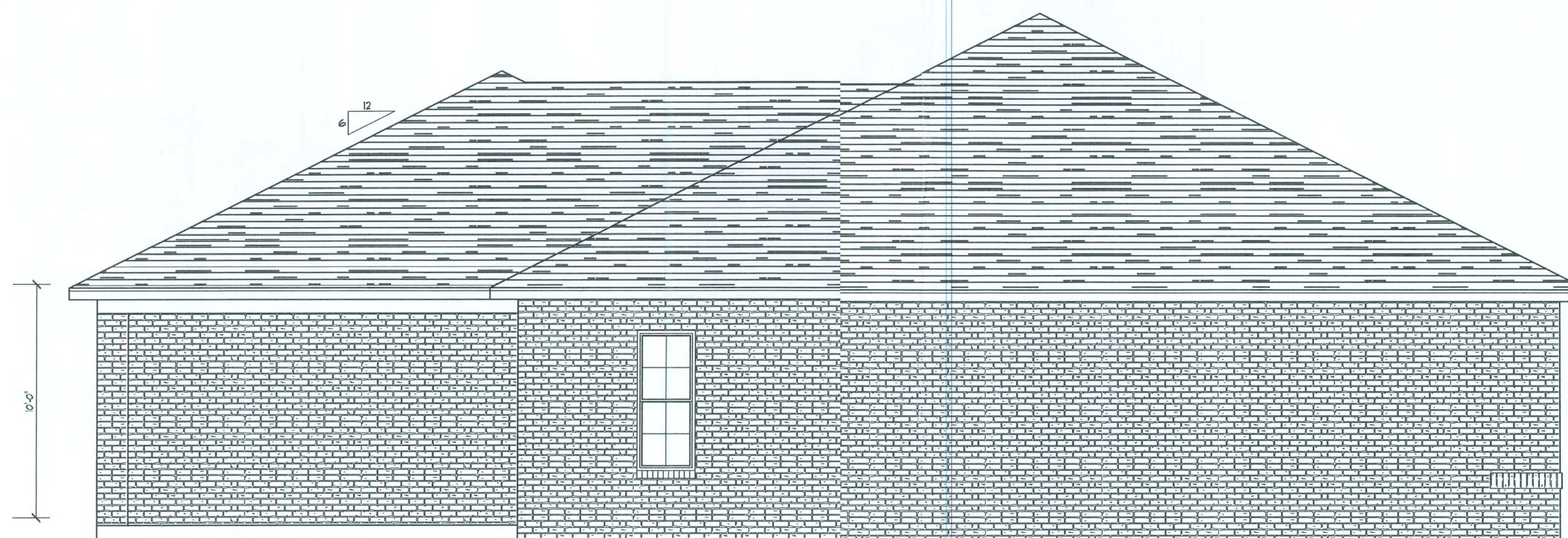
LEFT ELEVATION
