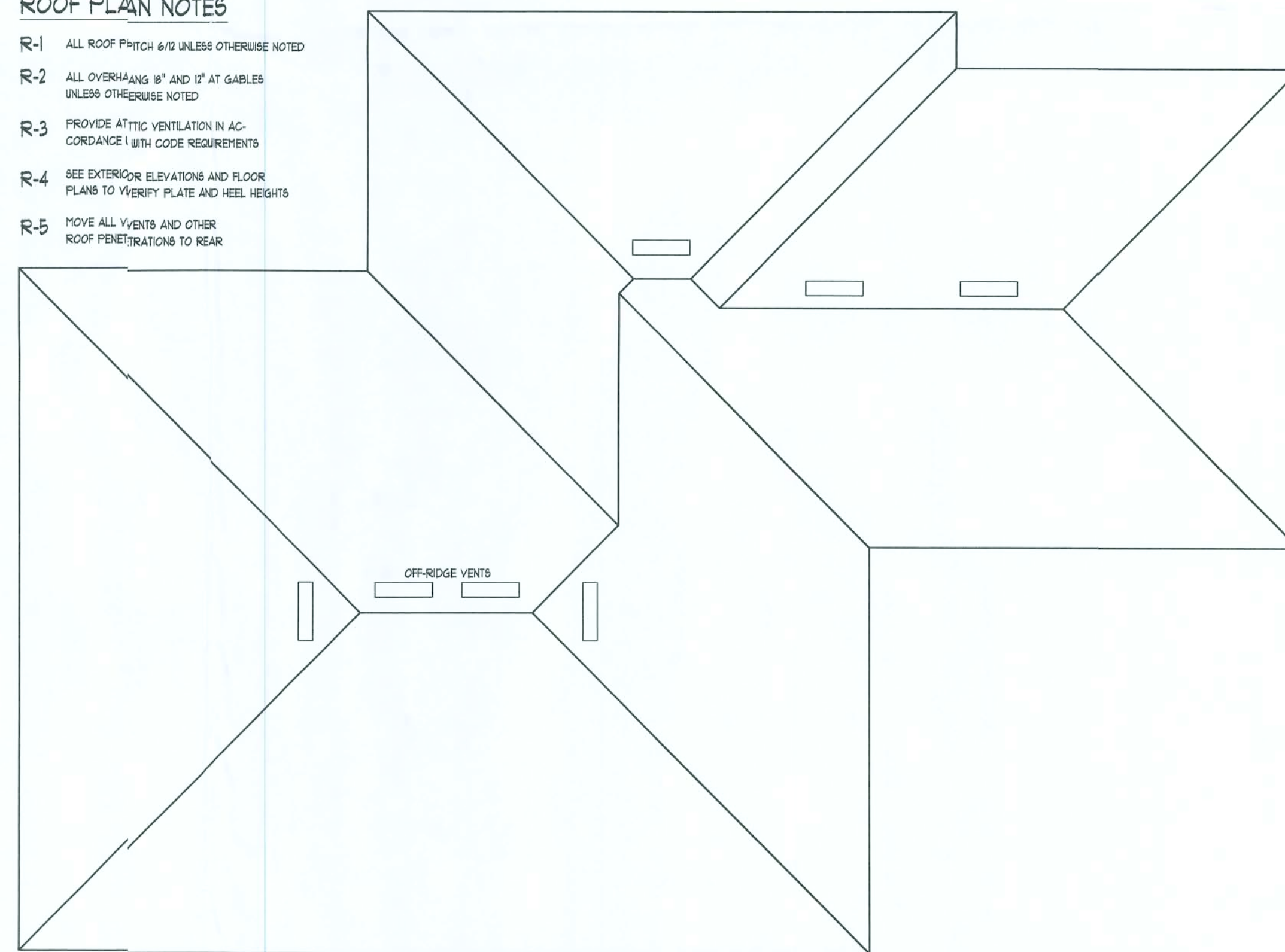
ROOF PLAN
