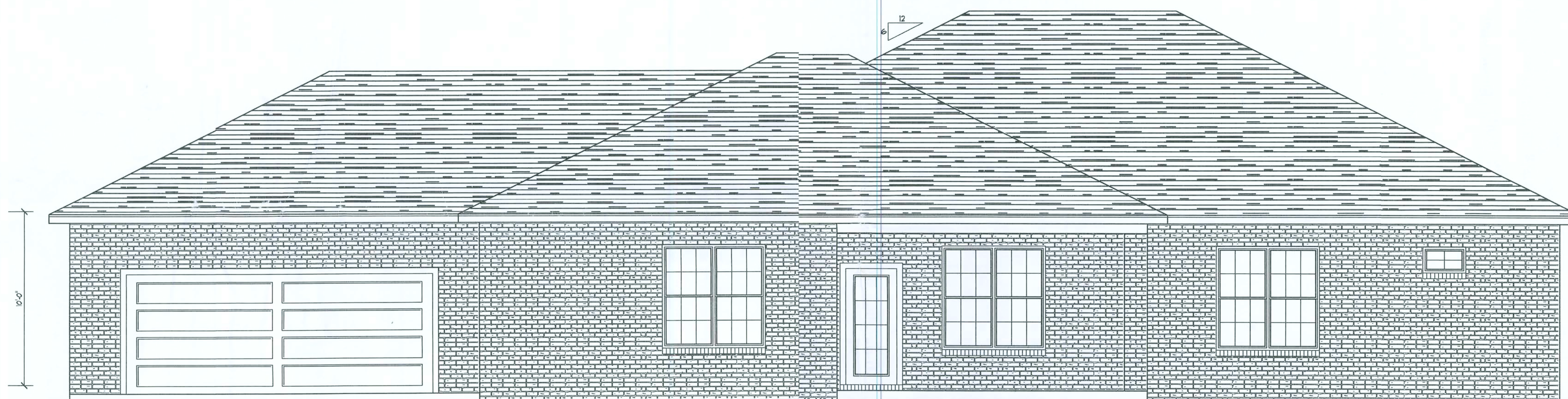
REAR ELEVATION
