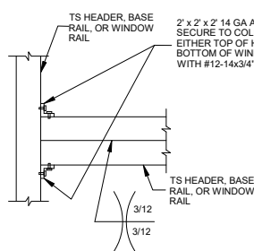
8B DOUBLE HEADER OR WINDOW RAIL TO POST CONNECTION DETAIL SCALE: NTS
