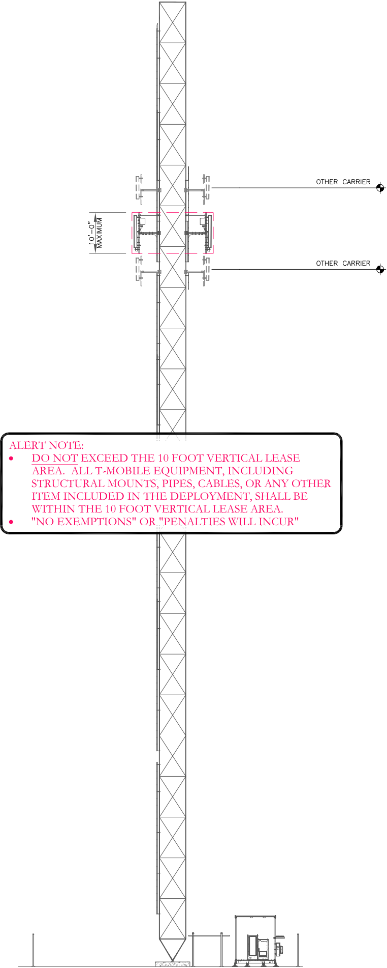
3 10 FOOT VERTICAL TOWER LEASE AREA SCALE: NOT TO SCALE
