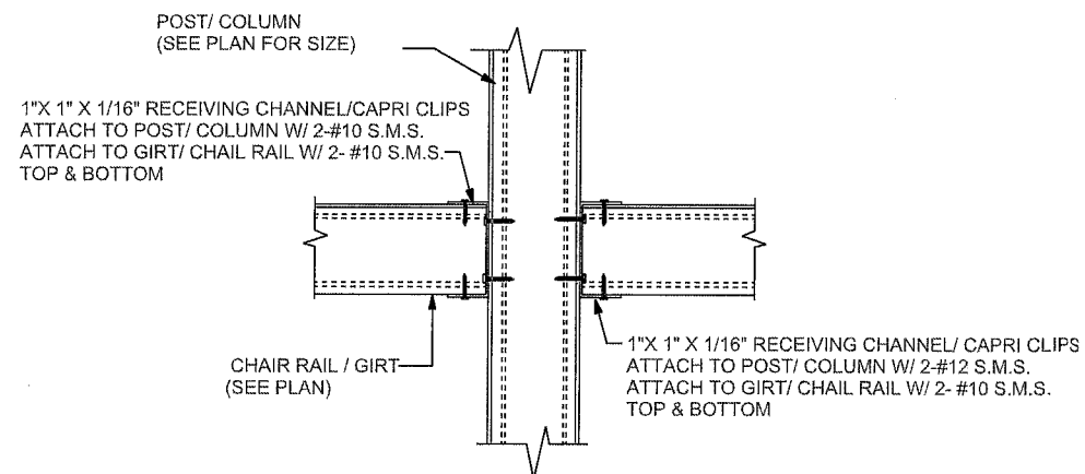
CHAIR RAIL TO POST/ COLUMN CONCEALED CONNECTION NTS
