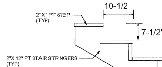
STAIR DETAIL
