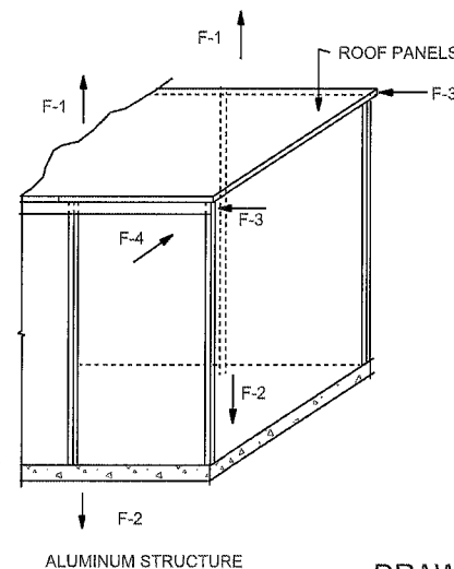
DRAWING L-1
