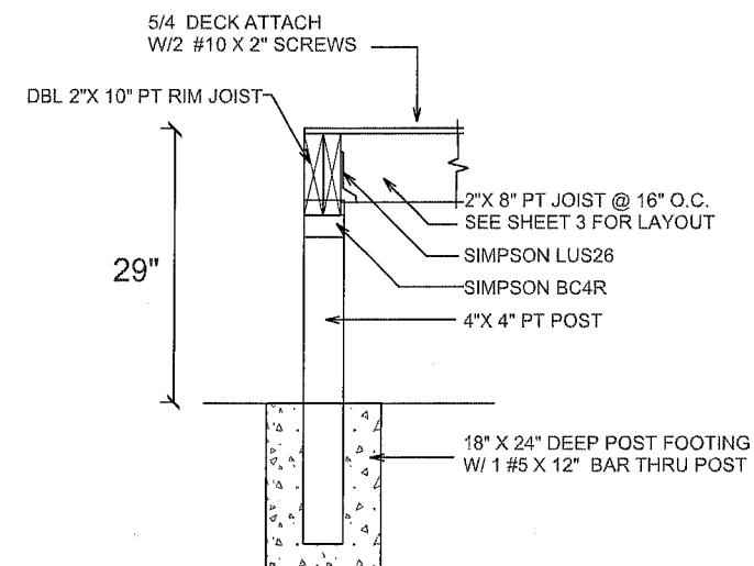
POST FOOTING TO DECK
