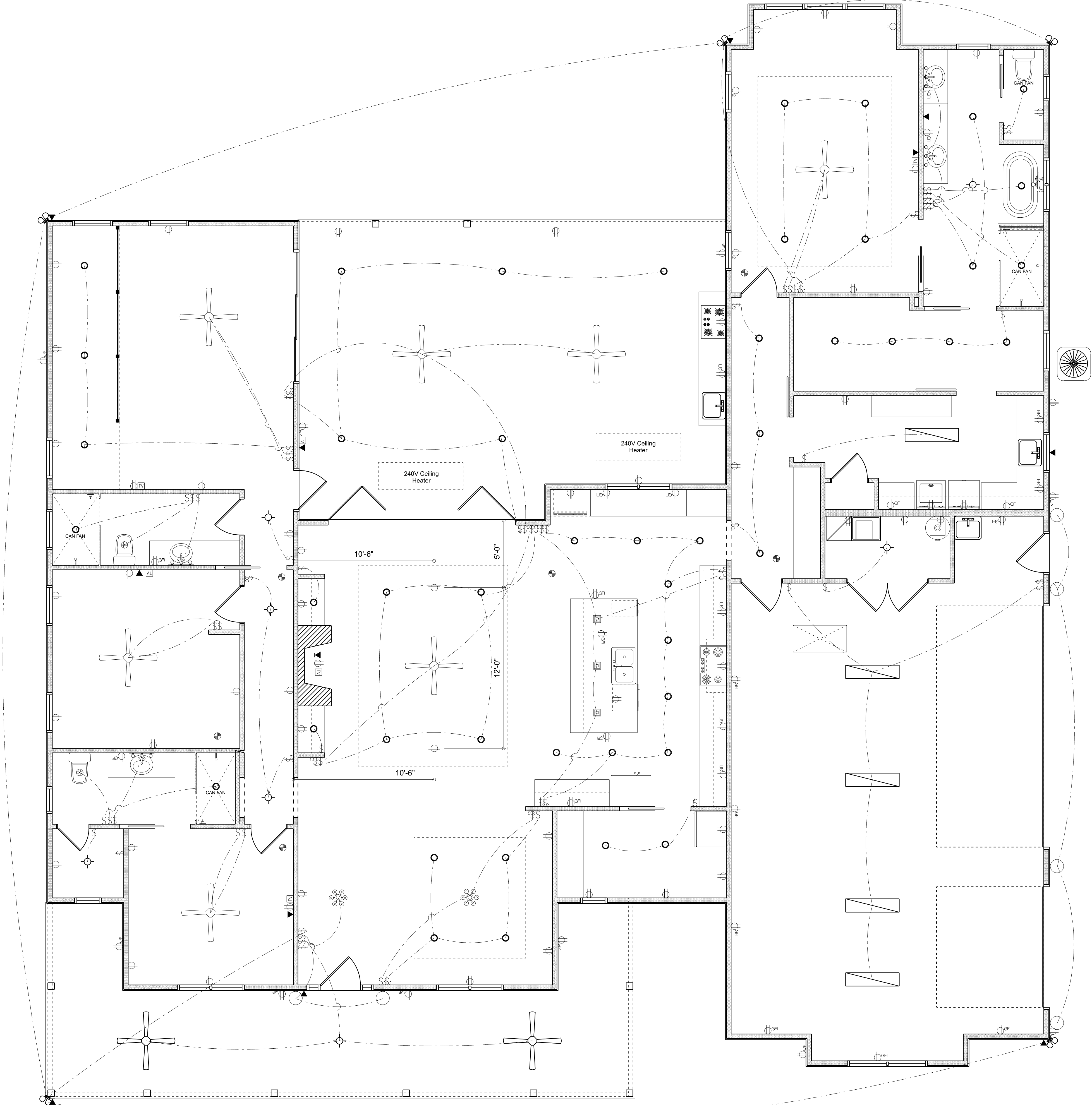
ELECTRICAL PLAN SCALE: 1/4" = 1'-0"
