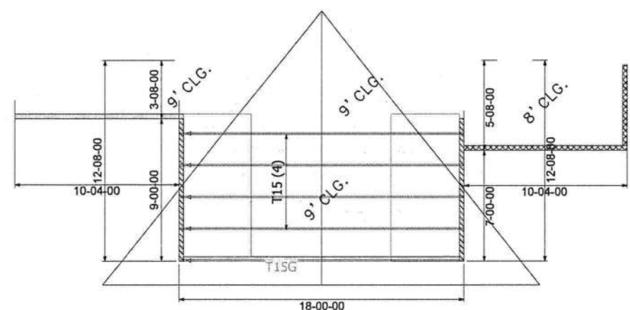
10/12 PITCH BONUS ROOM DORMER
