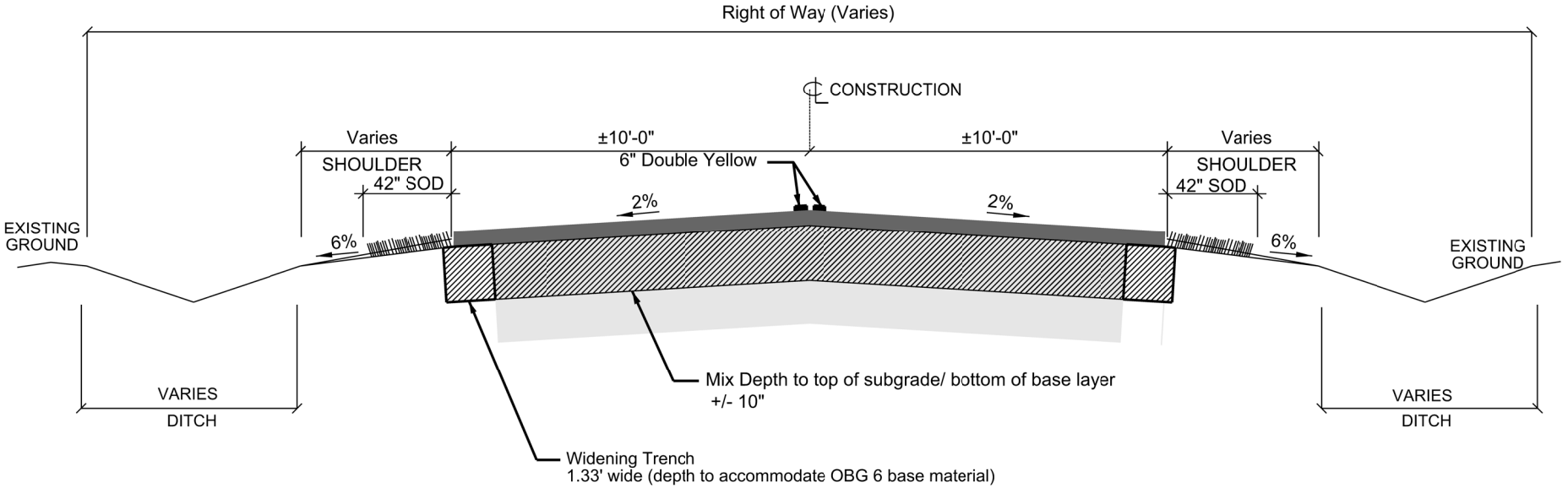
TYPICAL ROAD SECTION - N.T.S.
