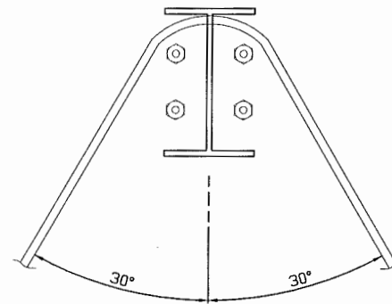
DETAIL 5
