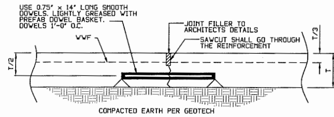
SAWCUT JOINT W/ DOWELS RECOMMENDED IF FORKLIFTS AND HEAVY TRAFFIC ARE USED.
