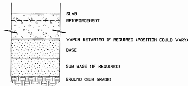
MAJOR COMPONENTS OF A SLAB ON GRADE SCALE: NOT A SCALE
