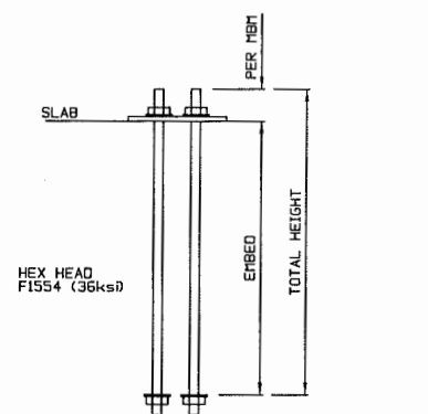
DETAIL 4
