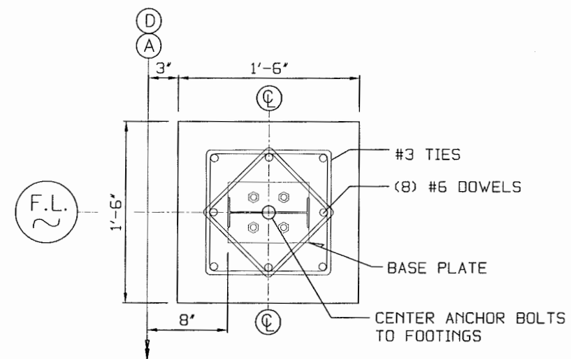
SECTION "RF"
