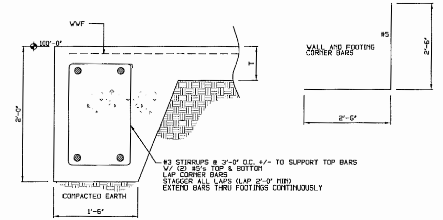
DETAIL 2A
