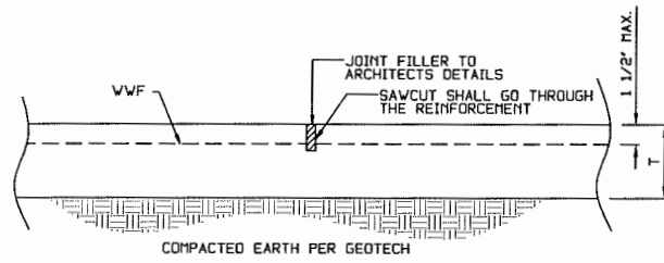
SAWCUT JOINT W/O DOWELS
