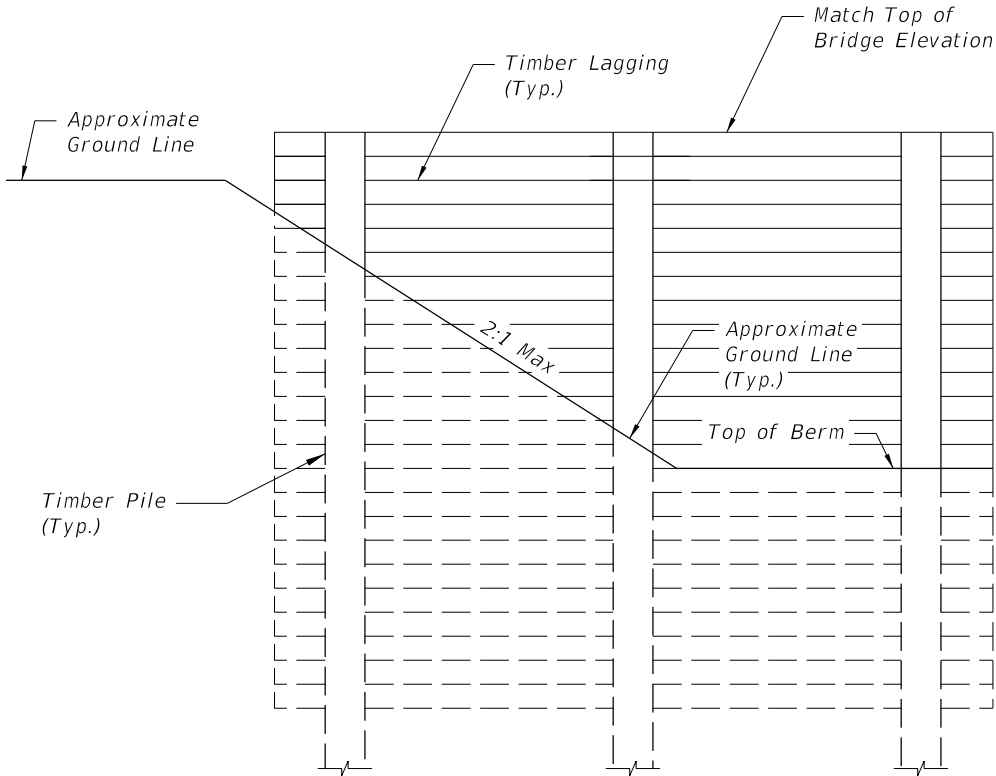
ELEVATION VIEW 1 - END BENT 9
