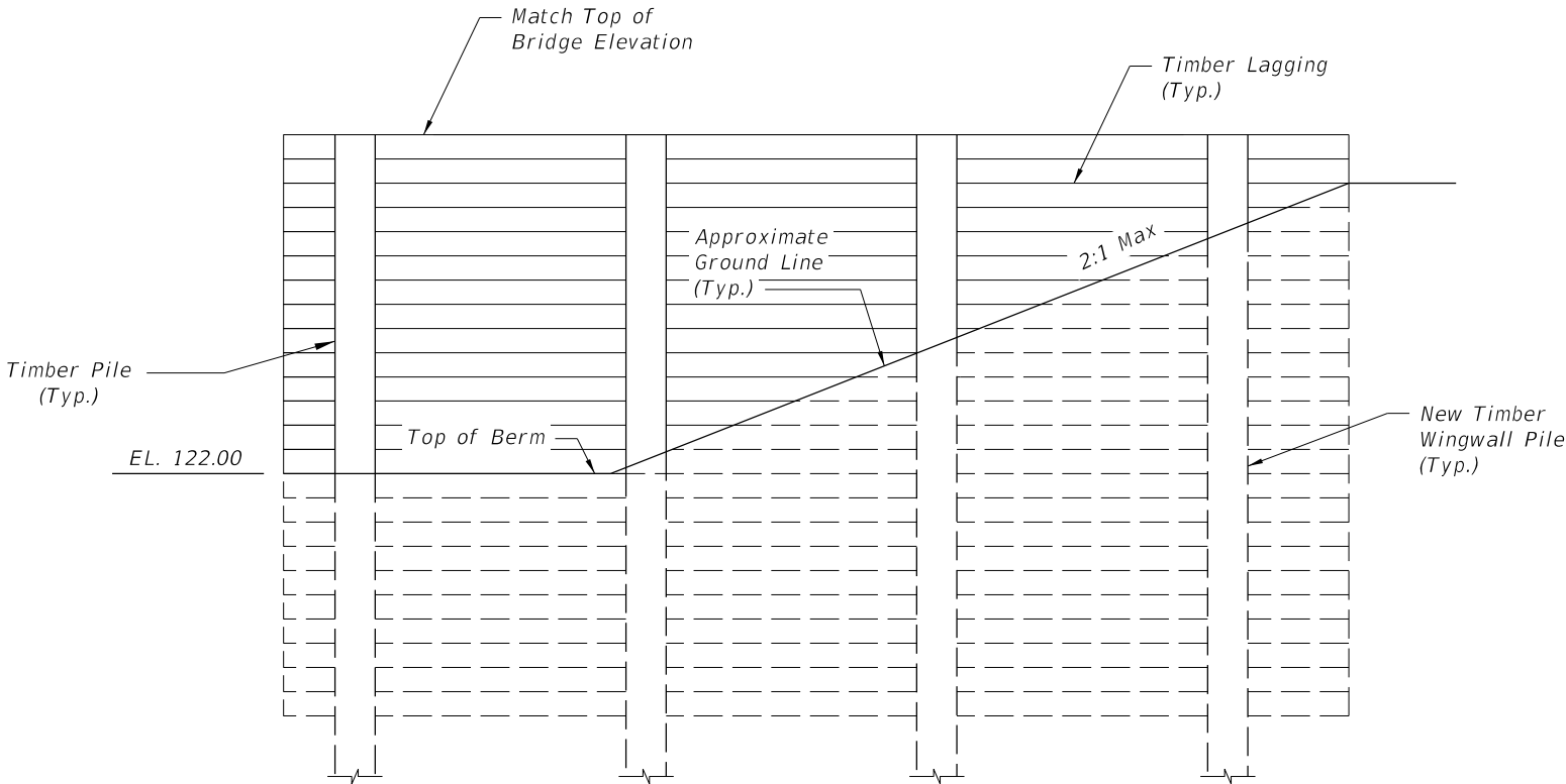
ELEVATION VIEW 3 - END BENT 9
