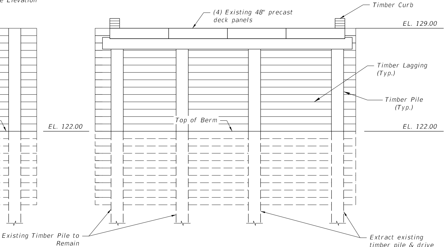
ELEVATION VIEW 2 - END BENT 9
