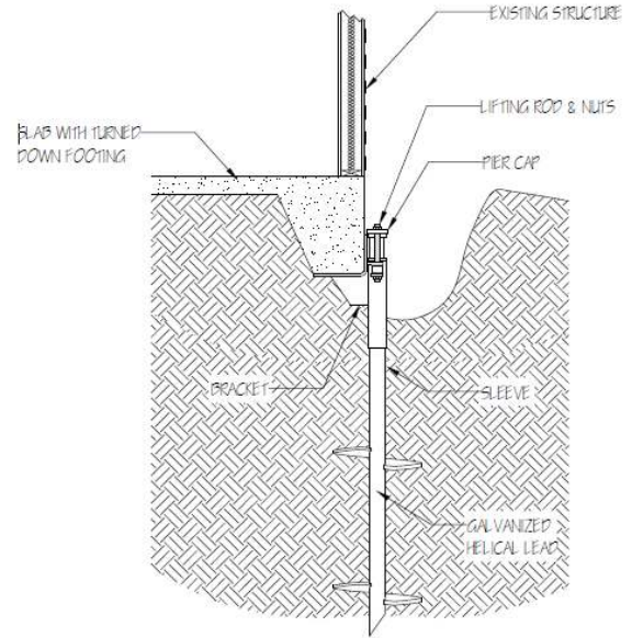
B 5001 HELICAL DETAIL 1/2" = 1' - 0"
