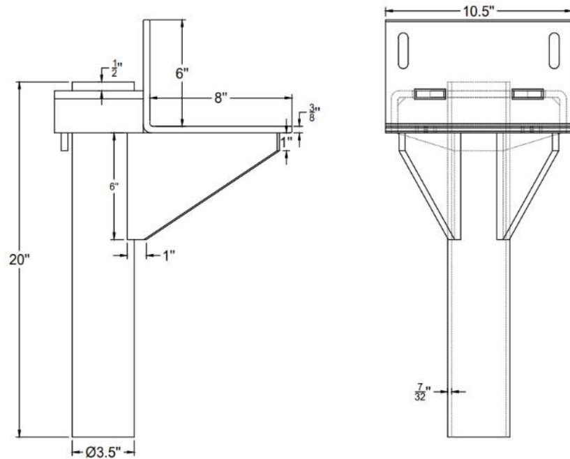
FIGURE A-5 – BRACKET (FRONT AND SIDE VIEW)
