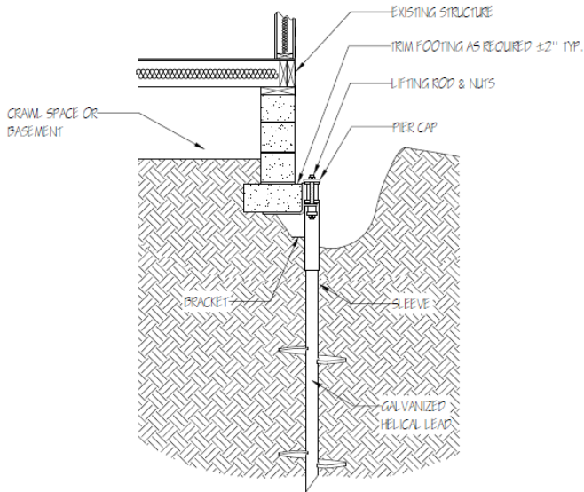
A 5001 HELICAL DETAIL 1/2" = 1' - 0"
