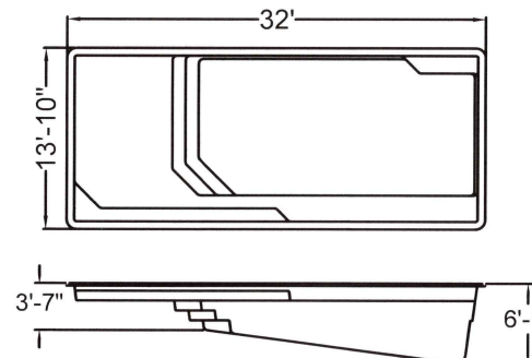
APOLLO 14 - CR14 7,700 gal. approx.
