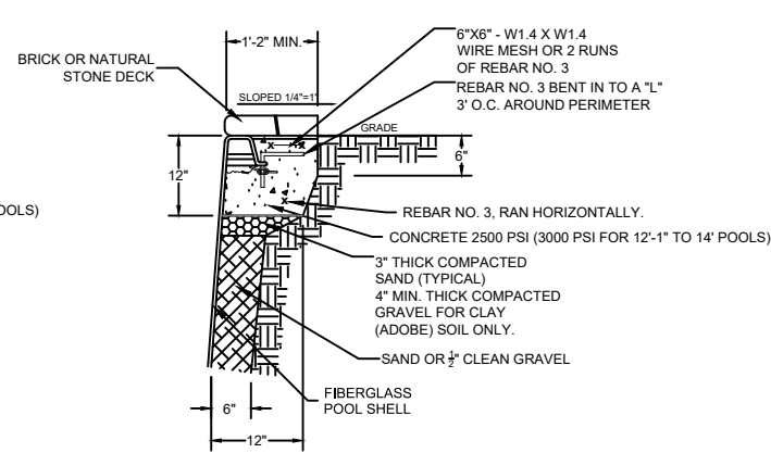
FIG. 7 CONCRETE DECK WITH BRICK OR STONE (For rectangle pools up to 12' wide or freeform pools up to 14' wide) (NOT FOR USE IN EXPANSIVE SOILS)
