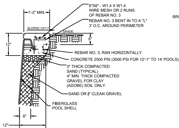
FIG. 6 TYPICAL CANTILEVER CONCRETE DECK (For rectangle pools up to 12' wide or freeform pools up to 14' wide) (NOT FOR USE IN EXPANSIVE SOILS)
