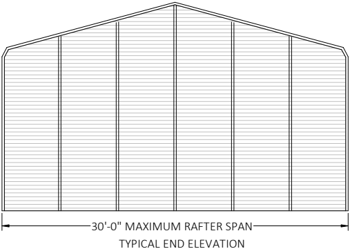
TYPICAL END ELEVATION
