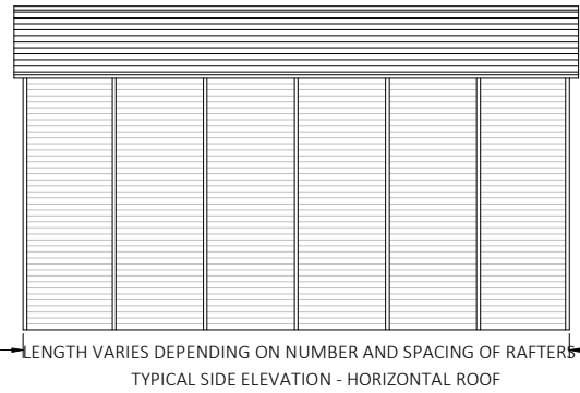
BOX EAVE FRAME RAFTER ENCLOSED BUILDING
