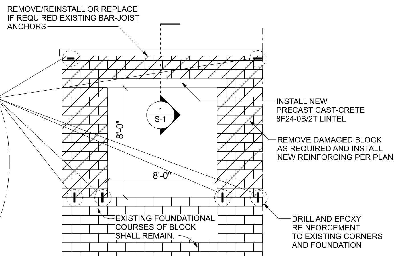
LOADING DOCK REPAIR SCALE: 1/4" = 1'-0"
