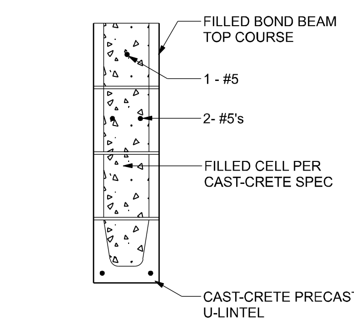
CAST-CRETE PRECAST LINTEL 8F24-0B/2T SCALE: NTS
