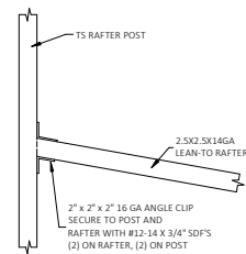
AFTER COLUMN CONNECTION DETAIL BRACE ON THE OTHER END OF THE RAFTER IS PER DETAIL 1.2/2 OR 1.2/3 BRACE ON THE OTHER END OF THE RAFTER IS PER DETAIL 1.1/2 OR 1.1/3 BRACE ON THE OTHER END OF THE RAFTER IS PER DETAIL 1/2 OR 1/3. SCALE: NTS
