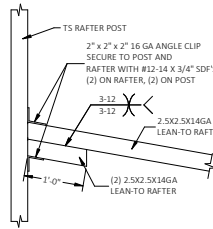
RAFTER COLUMN CONNECTION DETAIL KNEE BRACE ON THE OTHER END OF THE RAFTER IS PER DETAIL 1.2/2 OR 1.2/3 KNEE BRACE ON THE OTHER END OF THE RAFTER IS PER DETAIL 1.1/2 OR 1.1/3 KNEE BRACE ON THE OTHER END OF THE RAFTER IS PER DETAIL 1/2 OR 1/3. SCALE: NTS
