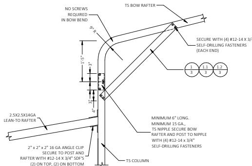
SIDE EXTENSION RAFTER/COLUMN DETAIL FOR EXTENSION RAFTER SPANS W' < 12'-0" , IF THE KNEE BRACE ON THE OTHER END OF THE RAFTER IS PER DETAIL 1.1/3; FOR EXTENSION RAFTER SPANS W' < 13'-0" , IF THE KNEE BRACE ON THE OTHER END OF THE RAFTER IS PER DETAIL 1.1/3; FOR EXTENSION RAFTER SPANS W' < 15'-0" , IF THE KNEE BRACE ON THE OTHER END OF THE RAFTER IS PER DETAIL 1/3; SCALE: NTS
