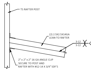
RAFTER COLUMN CONNECTION DETAIL KNEE BRACE ON THE OTHER END OF THE RAFTER IS PER DETAIL 1.2/2 OR 1.2/3 KNEE BRACE ON THE OTHER END OF THE RAFTER IS PER DETAIL 1.1/2 OR 1.1/3 KNEE BRACE ON THE OTHER END OF THE RAFTER IS PER DETAIL 1/2 OR 1/3. SCALE: NTS
