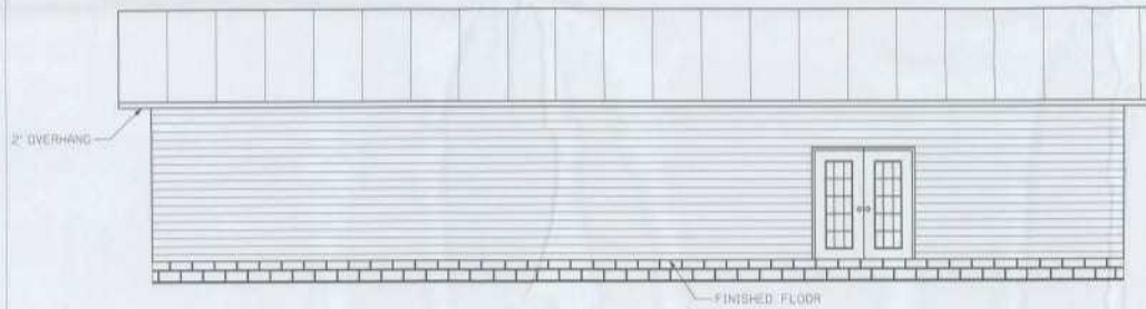
REAR ELEVATION
