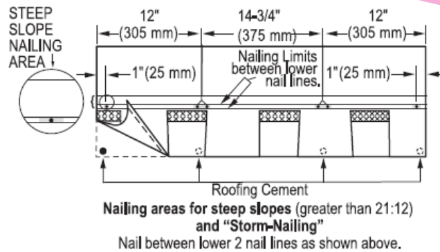
Six (6) Nail Attachment with Roofing Cement (> 21:12)
