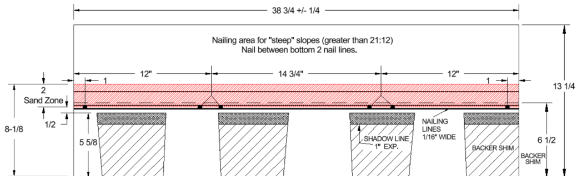
Typical view of Landmark, NorthGate and Patriot products with 2-inch Sand Zone
