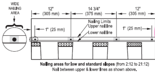
Four (4) Nail Attachment (2:12 to 21:12)
