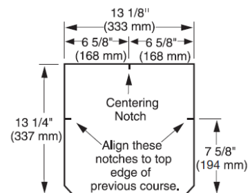
Shadow Ridge® ClimateFlex®
