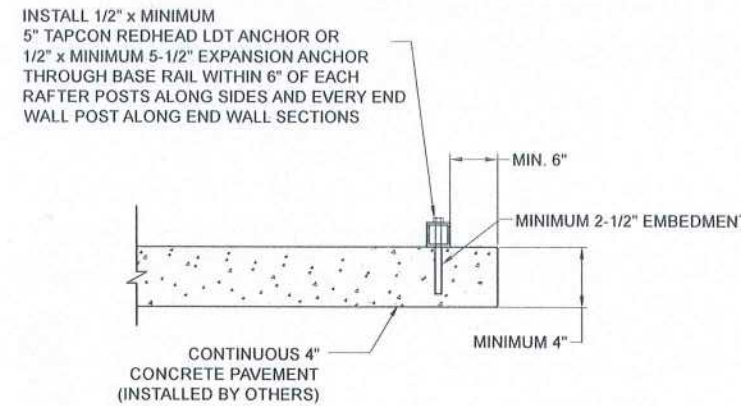
1B CONCRETE BASE RAIL ANCHORAGE Not To Scale (OPTIONAL - OPEN CARPORTS ONLY)
