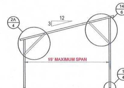
FREESTANDING LEAN-TO FRAMING PLAN NOT TO SCALE
