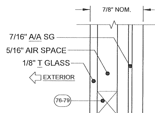
GLASS TYPE 14
