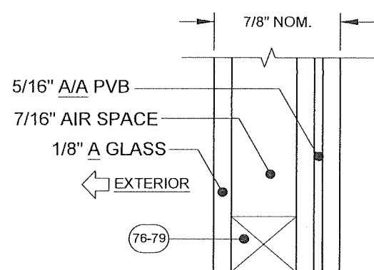
GLASS TYPE 5
