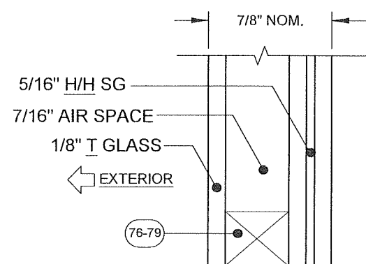
GLASS TYPE 10
