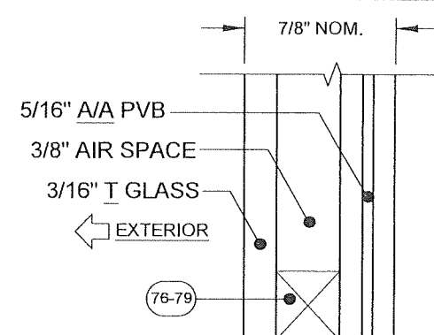
GLASS TYPE 8
