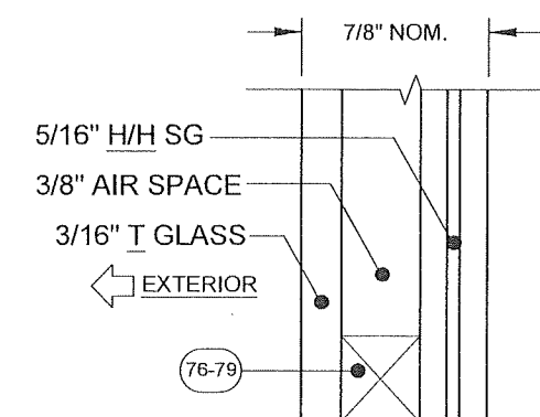
GLASS TYPE 12
