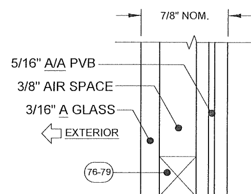
GLASS TYPE 7
