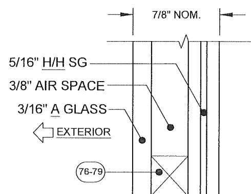
GLASS TYPE 11
