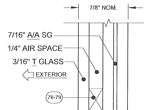
GLASS TYPE 16
