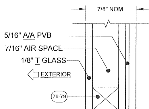
GLASS TYPE 6
