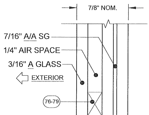
GLASS TYPE 15
