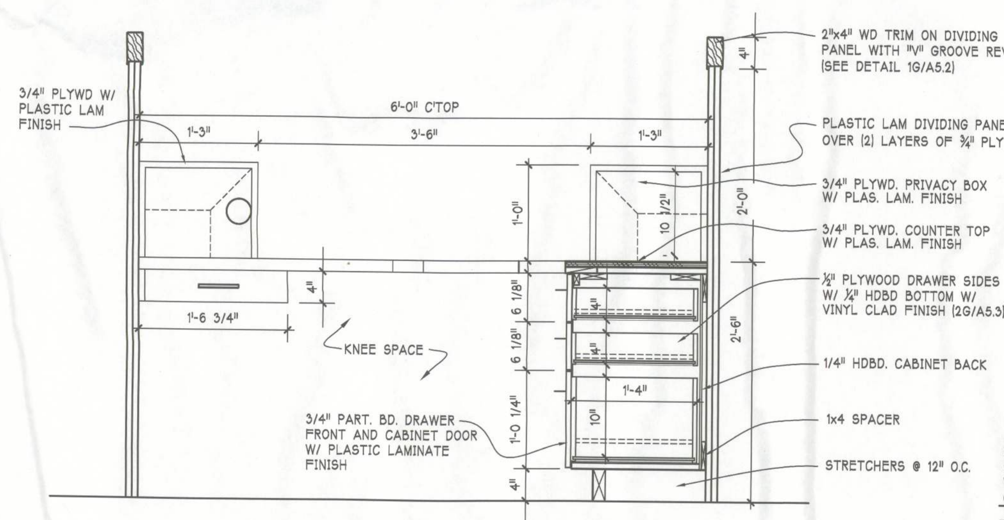
SECTION THRU CUSTOMER SERVICE STATION SCALE: 1" = 1'-0"
