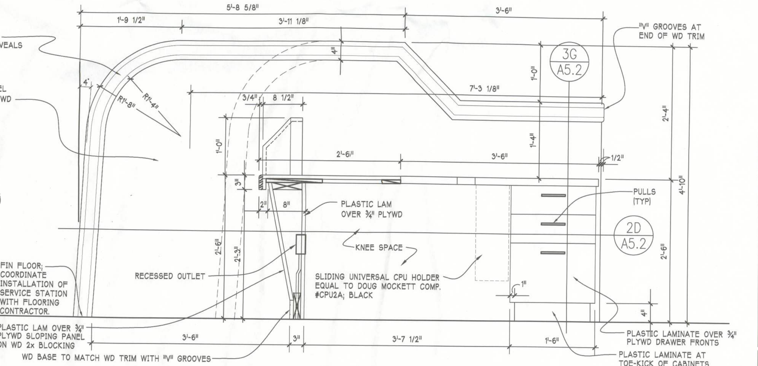
SECTION THRU CUSTOMER SERVICE STATION SCALE: 1" = 1'-0"
