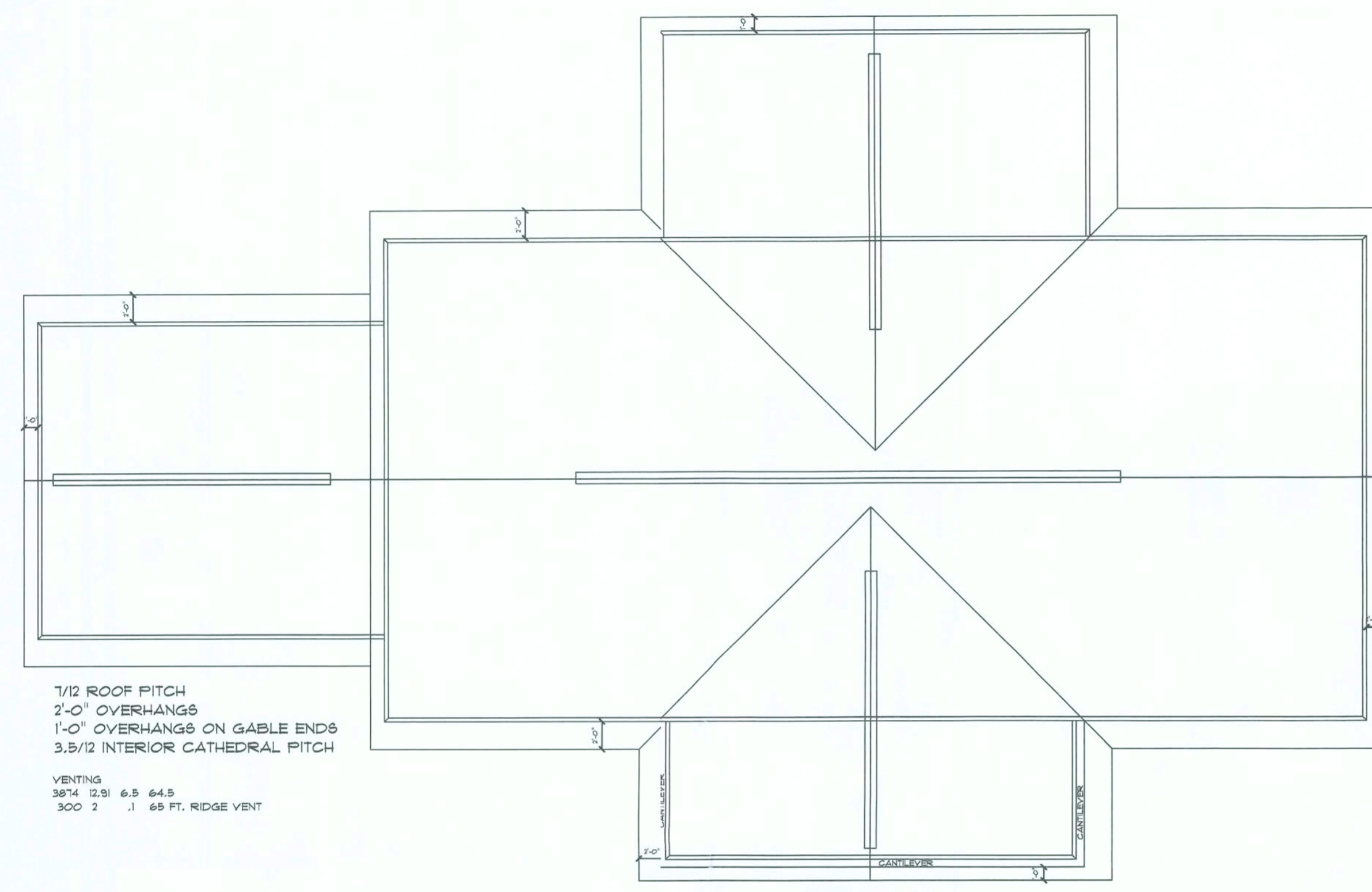
ROOF PLAN 1/8" SCALE
