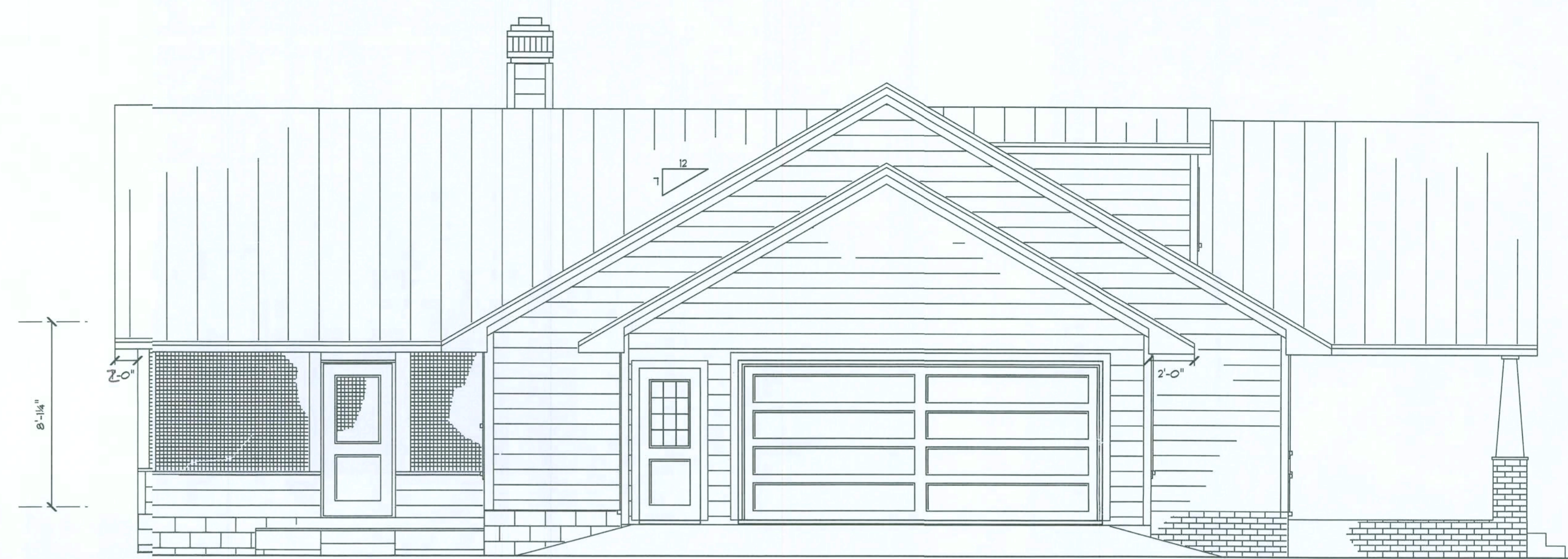
LEFT ELEVATION
