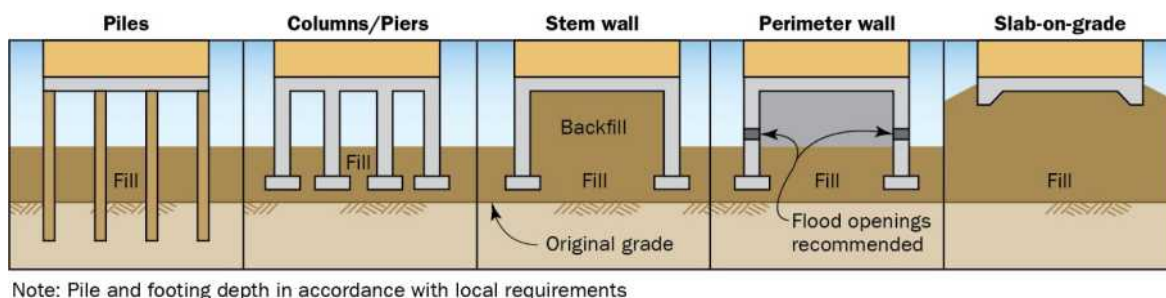
Figure 4: Non-basement foundation types
