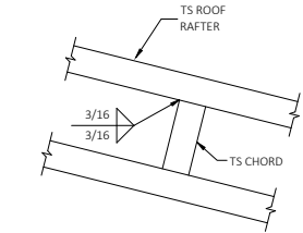
3 RAFTER TO CHORD CONNECTION SCALE: NTS
