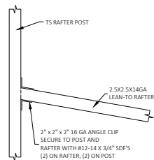
AFTER COLUMN CONNECTION DETAIL BRACE ON THE OTHER END OF THE RAFTER IS PER DETAIL 1.2/2 OR 1.2/3. BRACE ON THE OTHER END OF THE RAFTER IS PER DETAIL 1.1/2 OR 1.1/3. BRACE ON THE OTHER END OF THE RAFTER IS PER DETAIL 1/2 OR 1/3. SCALE: NTS
