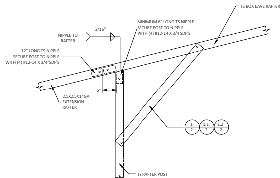
12'-0", IF THE KNEE BRACE ON THE OTHER END OF THE RAFTER IS PER DETAIL 1.2/2. 13'-0", IF THE KNEE BRACE ON THE OTHER END OF THE RAFTER IS PER DETAIL 1.1/2. 15'-0", IF THE KNEE BRACE ON THE OTHER END OF THE RAFTER IS PER DETAIL 1/2. SCALE: NTS
