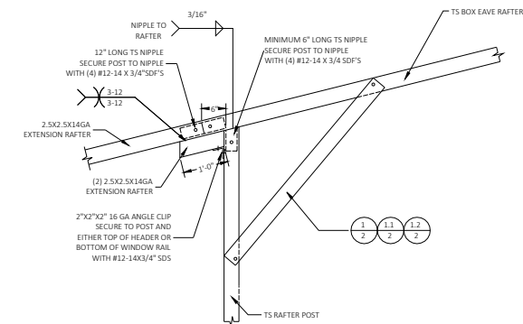
SIDE EXTENSION RAFTER/COLUMN DETAIL FOR EXTENSION RAFTER SPANS 12'-0" < W' <= 16'-0", IF THE KNEE BRACE ON THE OTHER END OF THE RAFTER IS PER DETAIL 1.2.2. FOR EXTENSION RAFTER SPANS 13'-0" < W' <= 18'-0", IF THE KNEE BRACE ON THE OTHER END OF THE RAFTER IS PER DETAIL 1.1/2. FOR EXTENSION RAFTER SPANS 15'-0" < W' <= 19'-0", IF THE KNEE BRACE ON THE OTHER END OF THE RAFTER IS PER DETAIL 1/2. SCALE: NTS
