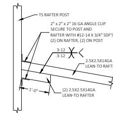
RAFTER COLUMN CONNECTION DETAIL KNEE BRACE ON THE OTHER END OF THE RAFTER IS PER DETAIL 1.2/2 OR 1.2/3. KNEE BRACE ON THE OTHER END OF THE RAFTER IS PER DETAIL 1.1/2 OR 1.1/3. KNEE BRACE ON THE OTHER END OF THE RAFTER IS PER DETAIL 1/2 OR 1/3. SCALE: NTS
