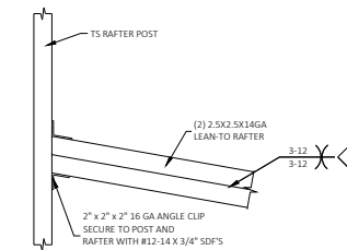
RAFTER COLUMN CONNECTION DETAIL KNEE BRACE ON THE OTHER END OF THE RAFTER IS PER DETAIL 1.2/2 OR 1.2/3. KNEE BRACE ON THE OTHER END OF THE RAFTER IS PER DETAIL 1.1/2 OR 1.1/3. KNEE BRACE ON THE OTHER END OF THE RAFTER IS PER DETAIL 1/2 OR 1/3. SCALE: NTS
