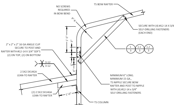
SIDE EXTENSION RAFTER/COLUMN DETAIL FOR EXTENSION RAFTER SPANS 12'-0" < W' <= 16'-0", IF THE KNEE BRACE ON THE OTHER END OF THE RAFTER IS PER DETAIL 1.2/3. FOR EXTENSION RAFTER SPANS 13'-0" < W' <= 18'-0", IF THE KNEE BRACE ON THE OTHER END OF THE RAFTER IS PER DETAIL 1.1/3. FOR EXTENSION RAFTER SPANS 15'-0" < W' <= 19'-0", IF THE KNEE BRACE ON THE OTHER END OF THE RAFTER IS PER DETAIL 1/3. SCALE: NTS
