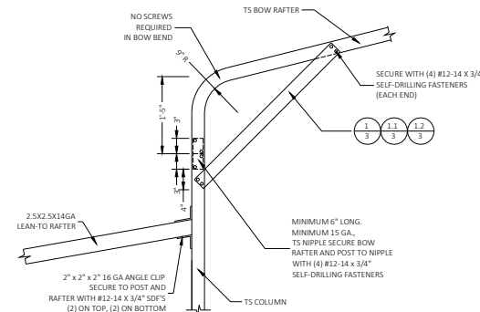
SIDE EXTENSION RAFTER/COLUMN DETAIL FOR EXTENSION RAFTER SPANS W' < 12'-0" , IF THE KNEE BRACE ON THE OTHER END OF THE RAFTER IS PER DETAIL 1.2/3. FOR EXTENSION RAFTER SPANS W' < 13'-0" , IF THE KNEE BRACE ON THE OTHER END OF THE RAFTER IS PER DETAIL 1.1/3. FOR EXTENSION RAFTER SPANS W' < 15'-0" , IF THE KNEE BRACE ON THE OTHER END OF THE RAFTER IS PER DETAIL 1/3. SCALE: NTS
