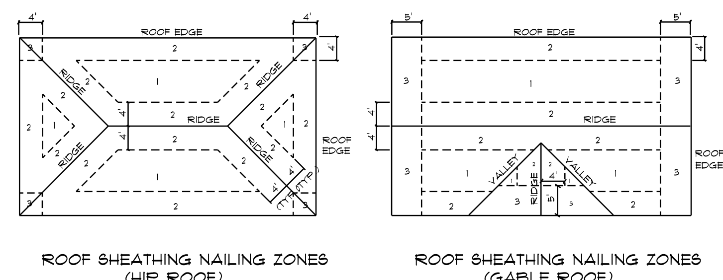
Roof Nail Pattern DET. SCALE: NONE B
