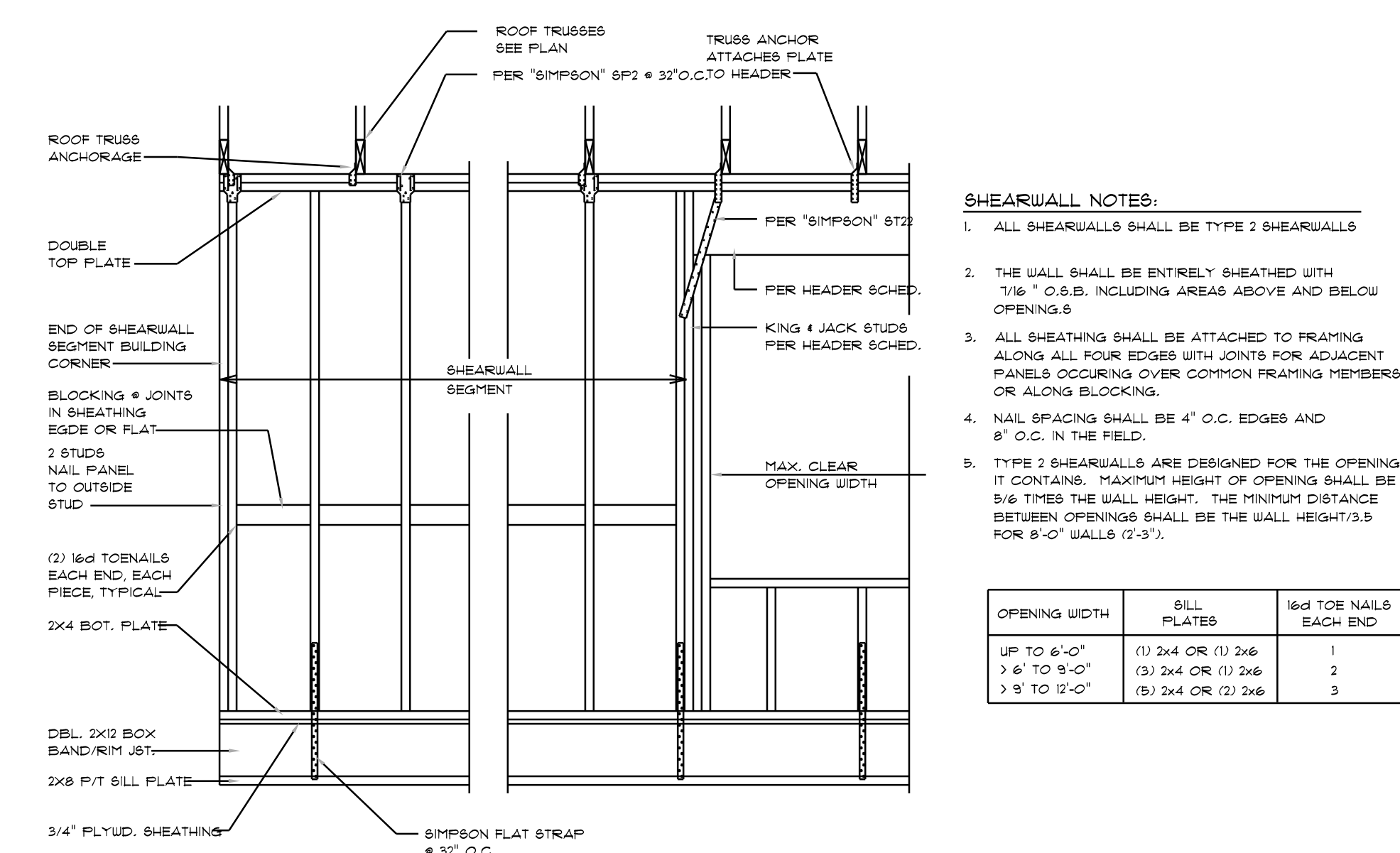
Shear Wall DETAILS SCALE: NONE J
