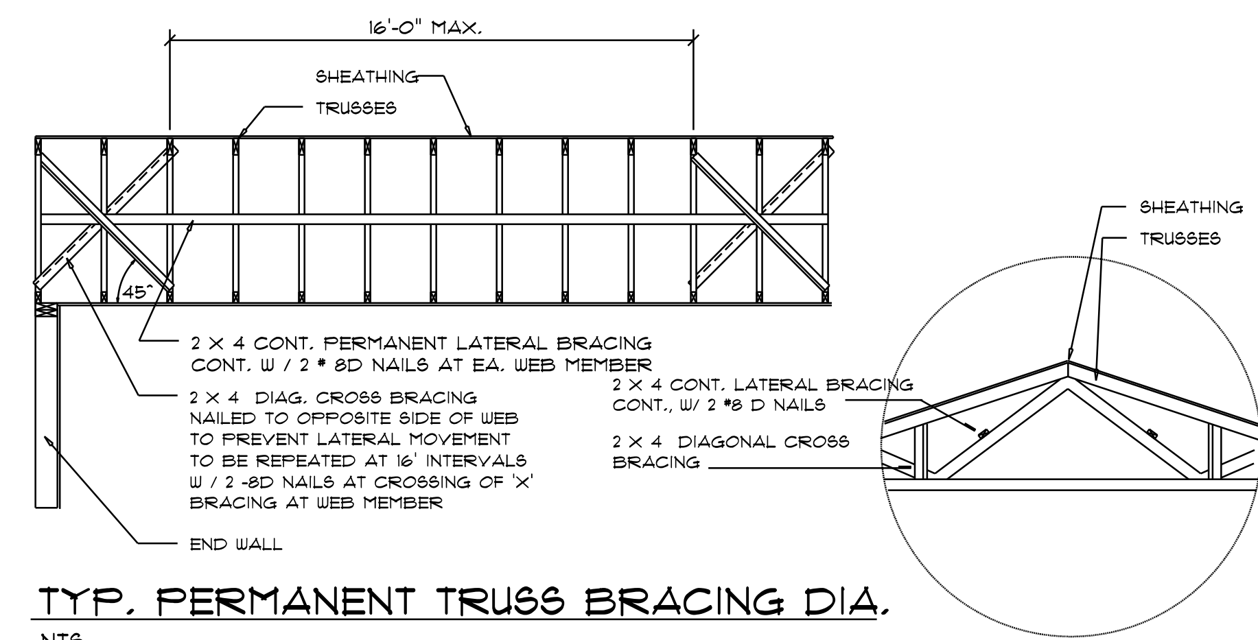
Truss Bracing DETAILS SCALE: AS NOTED D
