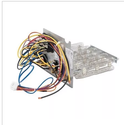
Factory Authorized Parts HTR KIT 5KW 230/1, 2-5T
